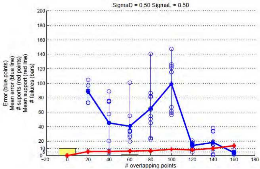
Fig. 9. SVD algorithm. The Gaussian noise is \sigma_D = \sigma_L = 0.50 .
