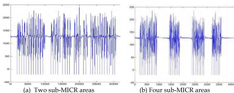
Fig. 3. MICR waveform
