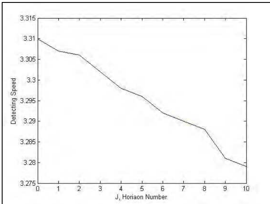
Fig. 24. Horizon versus fault-detecting speed for attenuating amplitude
