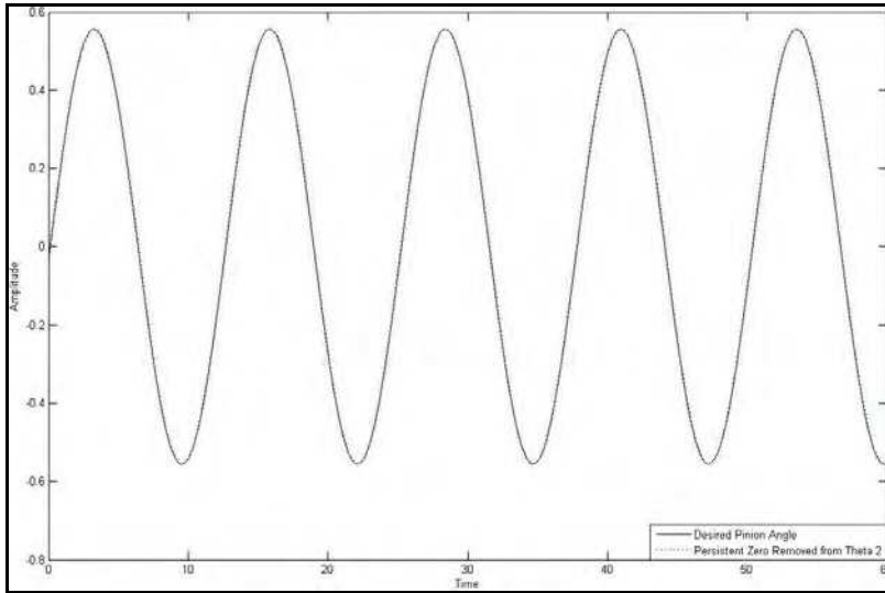
Fig. 21. Normal signal after persistent zero is removed
