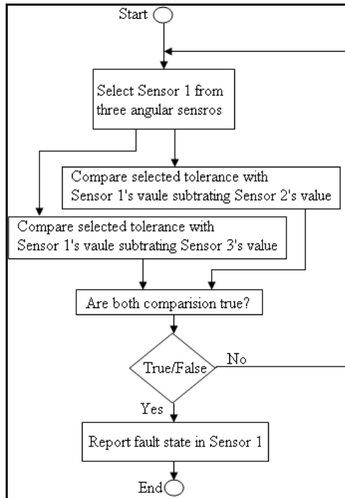
Fig. 8. Single-sensor FDIA logic
