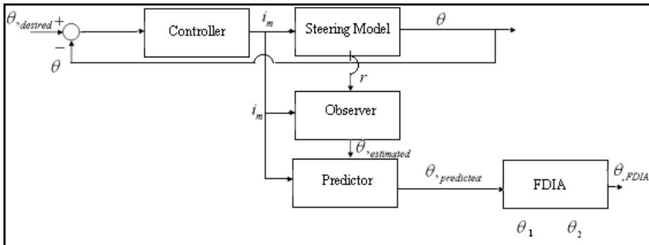
Fig. 15. Steering angle observation and predictor taken in SBW control system
