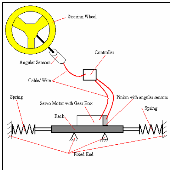
Fig. 1. Loop bench for simplified SBW system
