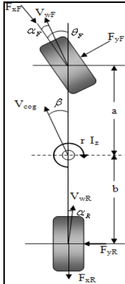
Fig. 6. Linear vehicle model simplified as bicycle model
