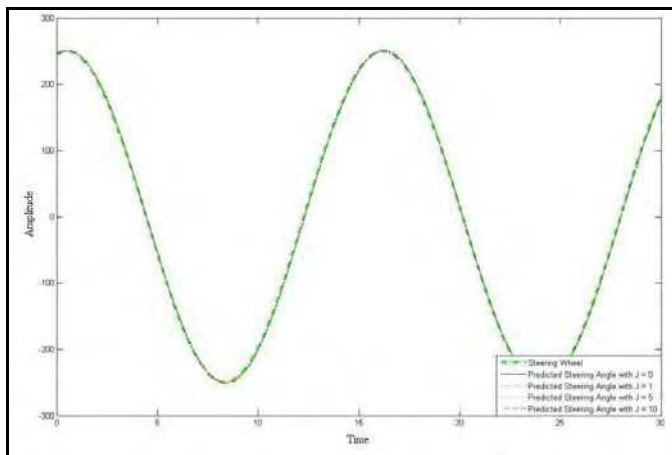
Fig. 16. Steering angle and estimated steering angle
