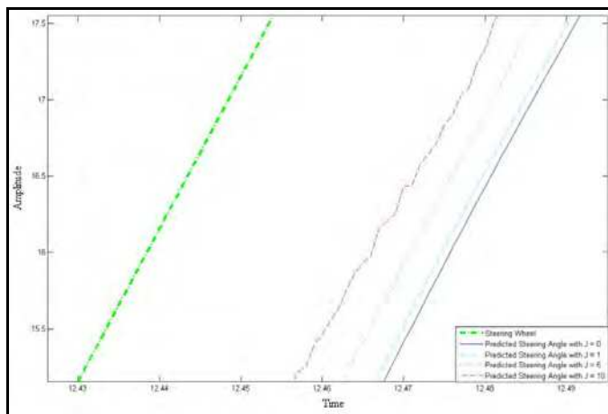
Fig. 17. A 0.04-second delay between \theta_{desired} and \theta_{estimated}
