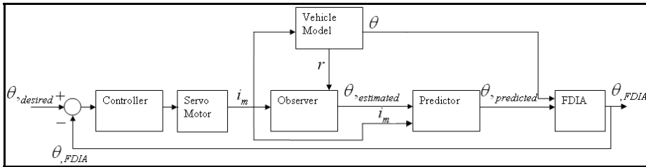
Fig. 3. Complete control model of simplified SBW system
