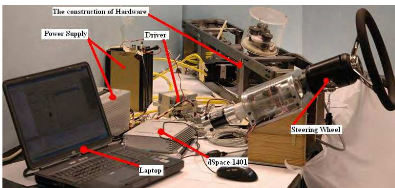
Fig. 5. Complete SBW hardware with all hardware components
