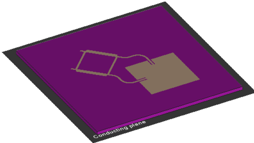
Fig. 13. The model of a RHC patch antenna with feed network.
