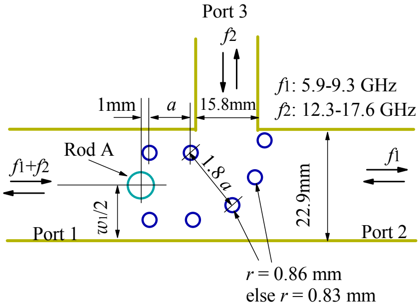
Fig. 12. Basic concept of the frequency multiplexer/demultiplexer.
