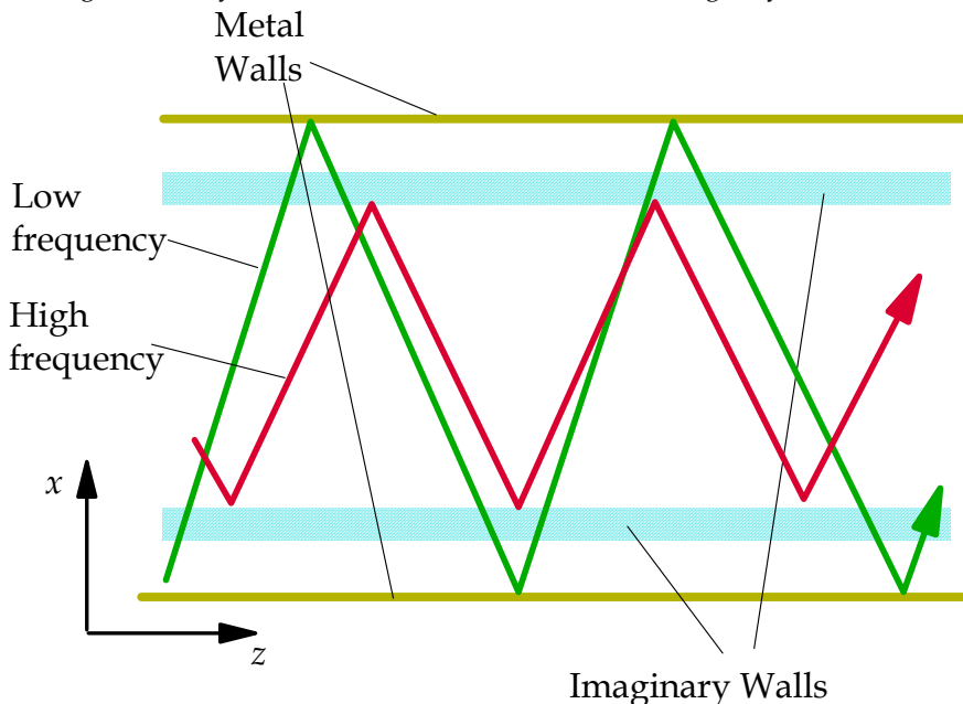
Fig. 1. Imaginary walls in a metallic waveguide.
