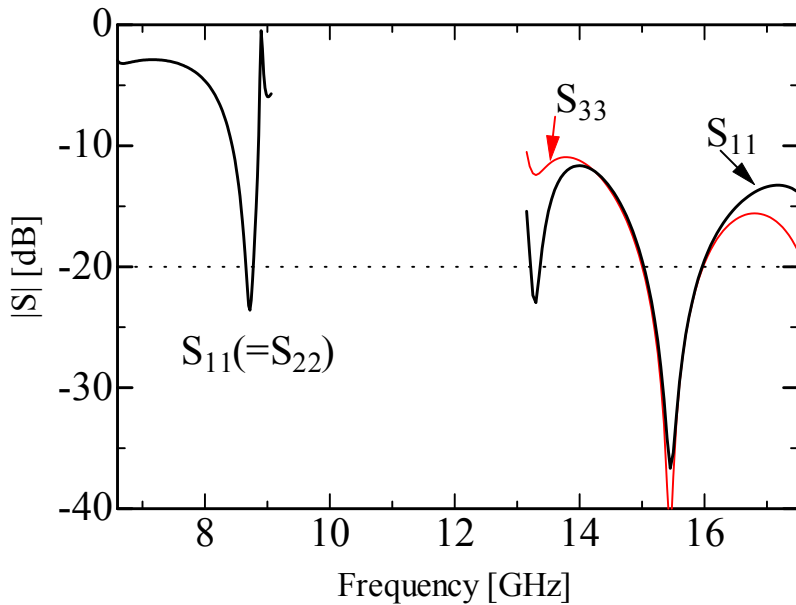
Fig. 13. Reflection coefficient |S_{11}| ( =|S_{22}| ) for low frequencies and |S_{11}| and |S_{33}| for high frequencies.
