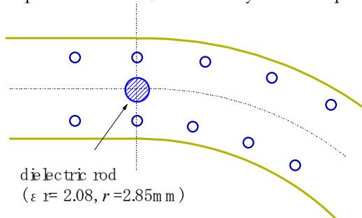
Fig. 7. Addition of another dielectric rod.
