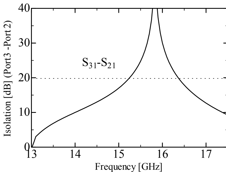
Fig. 15. Port isolation between two output ports.
