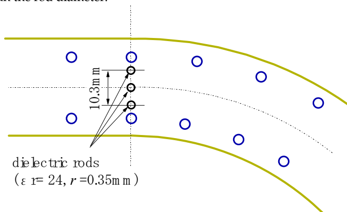
Fig. 10. Three thin \text{LaAlO}_3 rods that replace the thick Teflon rod shown in Fig.7
