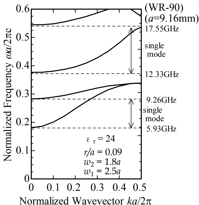
Fig. 4 Eigenvalue dispersion along the guide axis.
