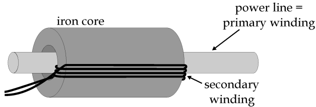
Fig. 7. The power pick-up device.
