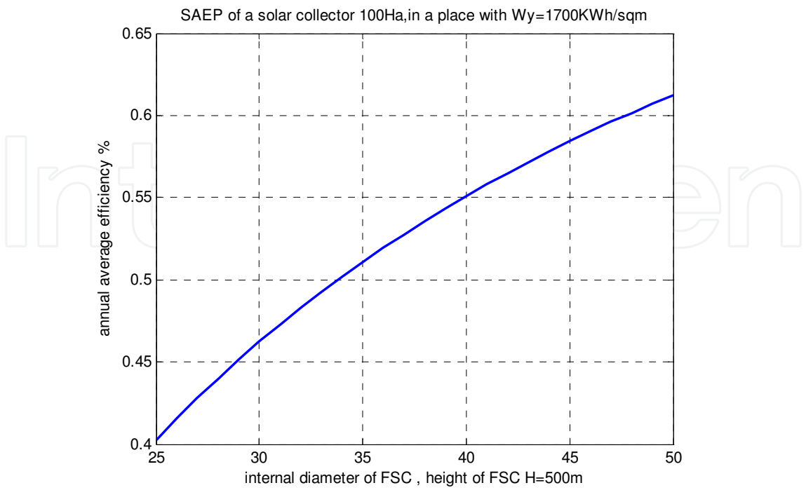
Fig. 6. variation of the annual efficiency of a SAEP with internal FSC diameter
