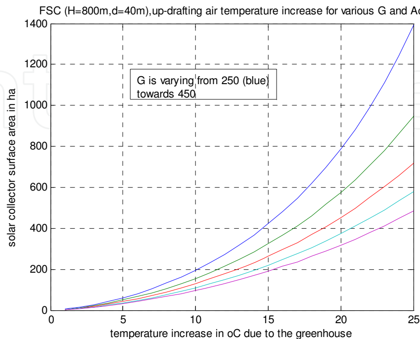
Fig. 11. The solar collector area as a function of its generating temperature increase Example: for a solar collector of surface area A_c=400\text{Ha} (i.e. 400000\text{m}^2 ), with a diameter D_c\approx 715\text{m} , for an equivalent horizontal solar irradiance G of 250\text{W/m}^2 , the created temperature difference \Delta T is \sim 14.5^\circ\text{C} and the free up-drafting air speed v inside the FSC of H=800\text{m} height and d=40\text{m} internal diameter will be \sim 21\text{m/sec} , while for G=450\text{W/m}^2 , \Delta T is \sim 22.5^\circ\text{C} and v is \sim 27\text{m/sec} . For one dimensional analysis a\approx 1 and if the friction losses are negligible, i.e. k\approx 0 , we have:
