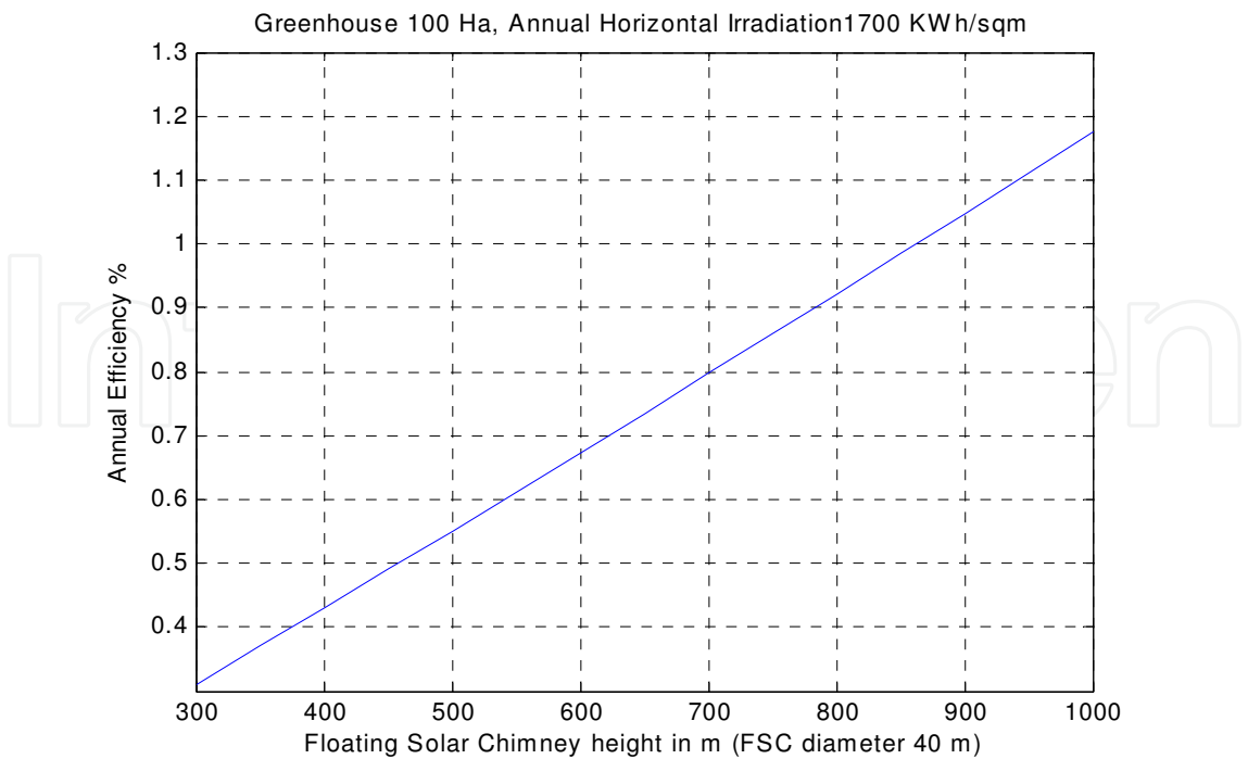
Fig. 5. Annual efficiency of a SAEP as function of its FSC height height H , the annual generated electricity by the SAEPs is also proportional to the Floating Solar Chimney height H , is as follows:
