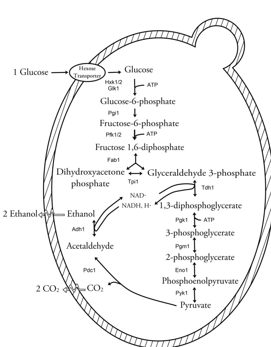
Figure 1. Glycolysis and alcoholic fermentation steps on S. cerevisiae (adapted from [23]).
