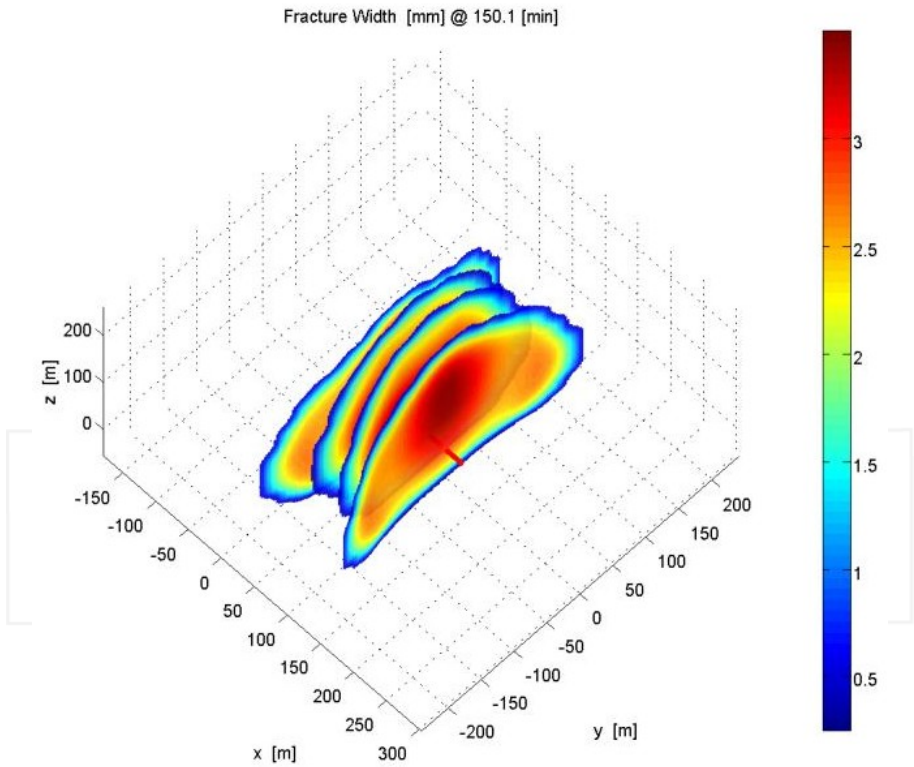
Figure 8. Fracture geometry with high viscosity frac fluid at 150 mins
