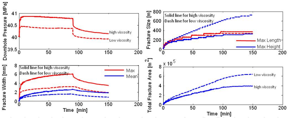
Figure 7. Calculated fracture parameters
