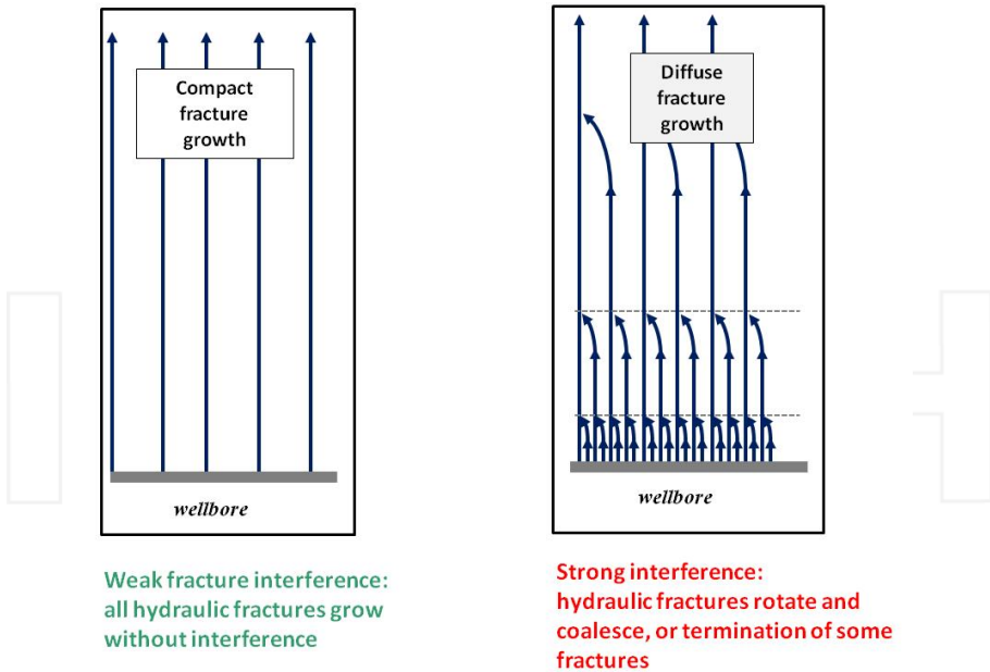
Figure 1. "Compact" and "Diffuse" fracture growth patterns
