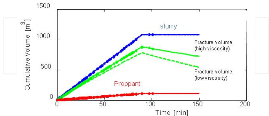
Figure 6. Injection volume and calculated fracture volumes
