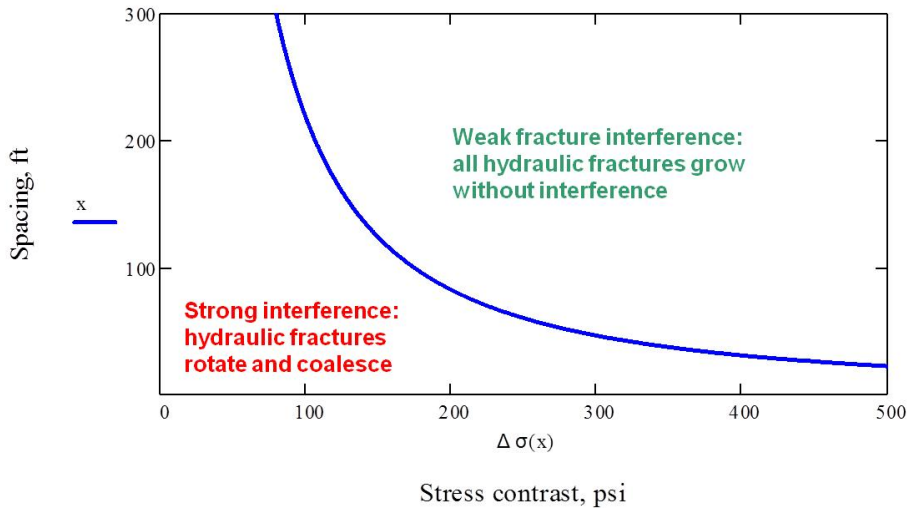
Figure 3. Fracture spacing versus stress contrast
