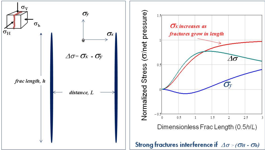
Figure 2. Interaction between two fractures
