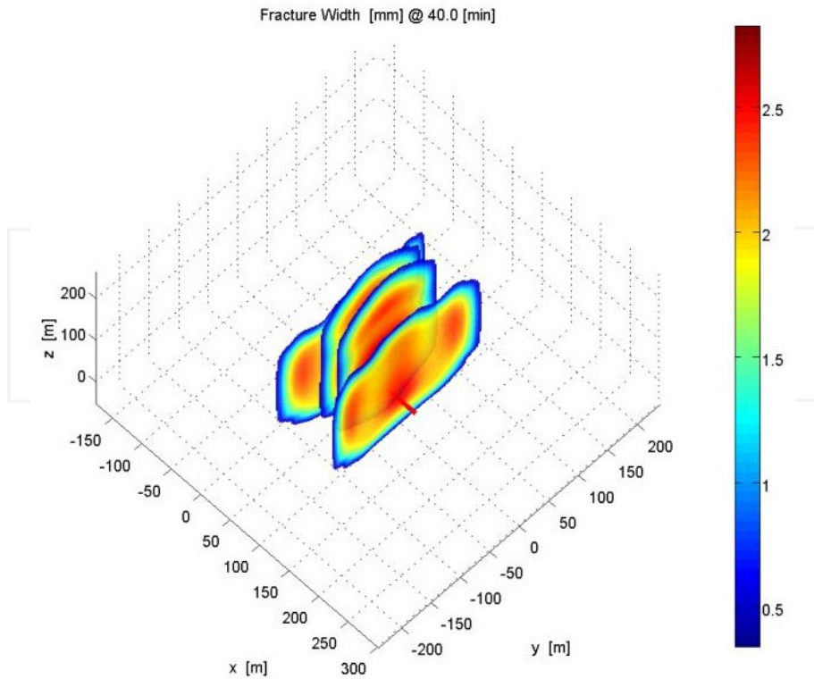
Figure 11. Fracture geometry of low viscosity frac fluid after 40 mins
