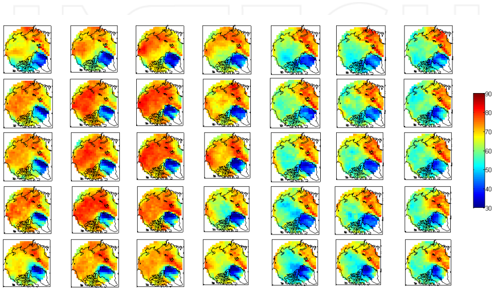
Figure 3. Node- averaged cloud fraction (in %) ascribed to a corresponding SLP pattern of the master SOM.
