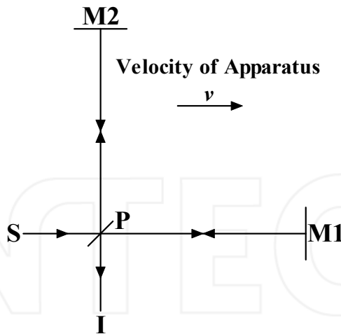
Figure 2. Michelson-Morley Experiment
