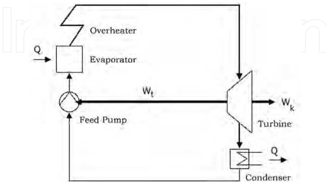
Fig. 6. Thermal dynamic flowchart of the closed Rankine cycle process.
