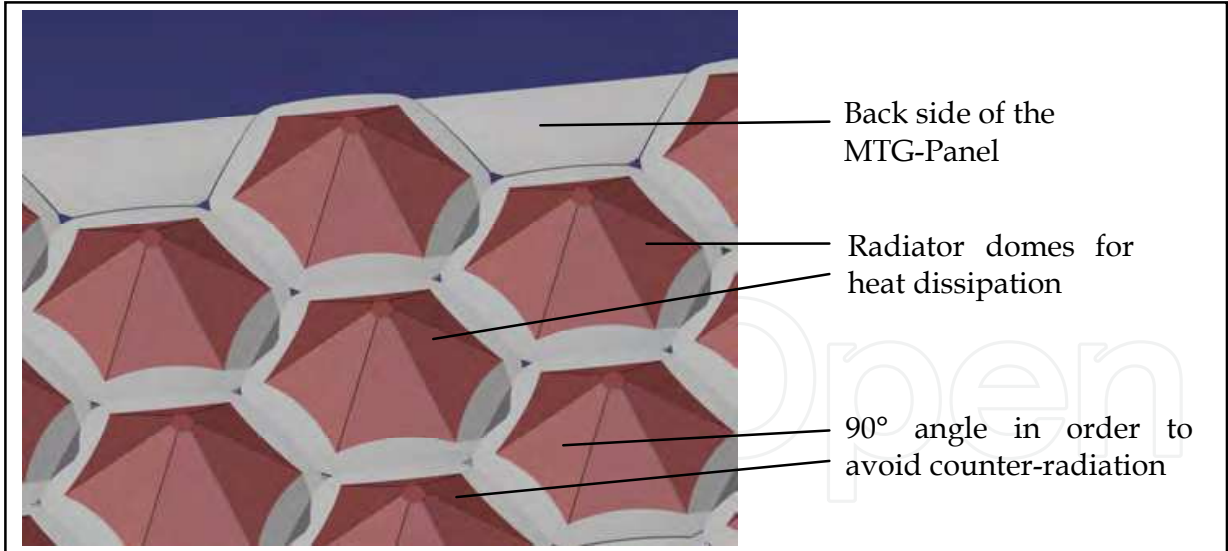
Fig. 10. Key principle for the condenser/ radiator, where radiation domes shall optimize the radiation area, the opposite radiator plates always stand with an angle of 90° to each other in order to avoid counter-radiation
