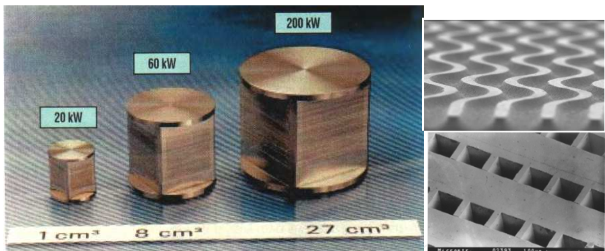
Fig. 8. Different microstructure heat exchanger made of stainless steel, each channel at 100µm edge length; (Brandner & Schubert, 2005)
