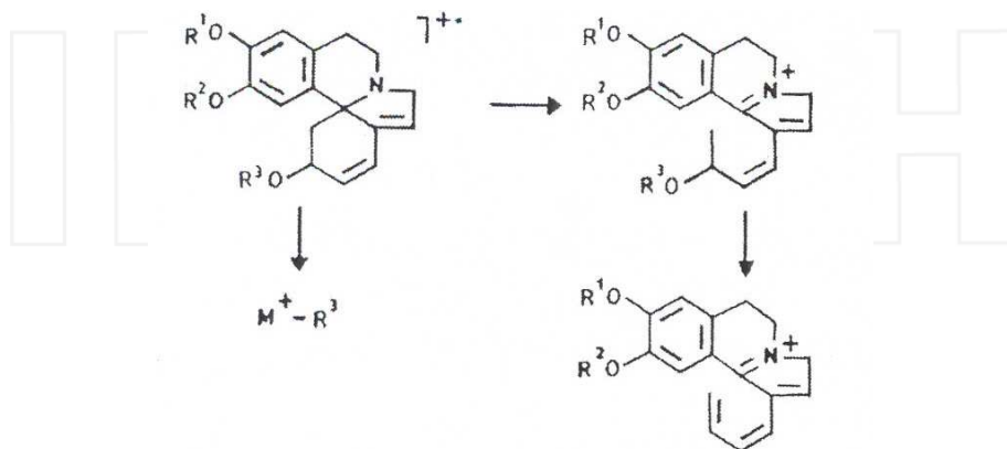
Fig. 3. Fragmentation of dienoid alkaloids
