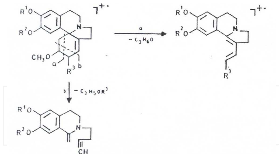
Fig. 4. Fragmentation of the alkenoid alkaloids
