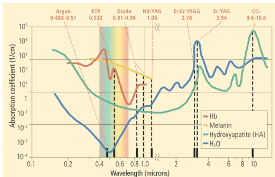
Fig. 3. Absorption curve of various tissue components.
