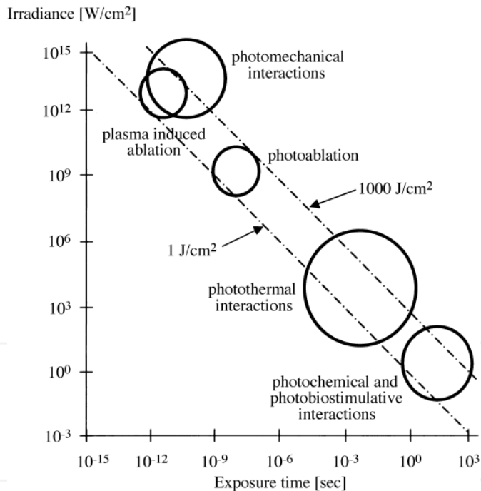
Fig. 4. Representation of laser-tissue interactions in terms of exposure time and irradiance
