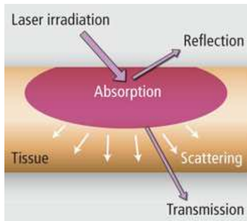
Fig. 2. What happens when Laser hits the tissue?
