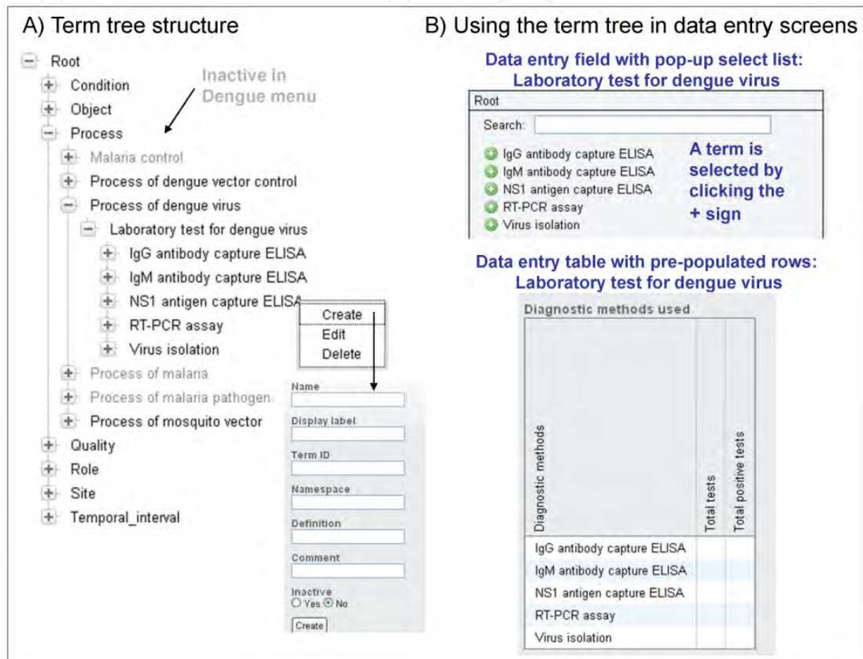
Fig. 3. Partially opened term tree structure for dengue menu and use of configurable term tree lists in data entry screens. A) Example of term tree section leading to laboratory tests for dengue virus. B) Using the term tree section for laboratory tests for dengue virus in data entry fields and tables. Adapted from a figure presented previously by L. Eisen et al. (2011).
