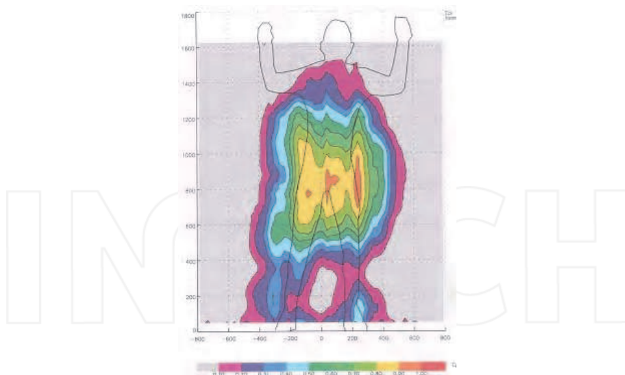
Fig. 14. Mapping of the air flow behind a cross country skier (Wind tunnel of IAT, France). The more colours are warm, the more the aerodynamic resistance is important.
