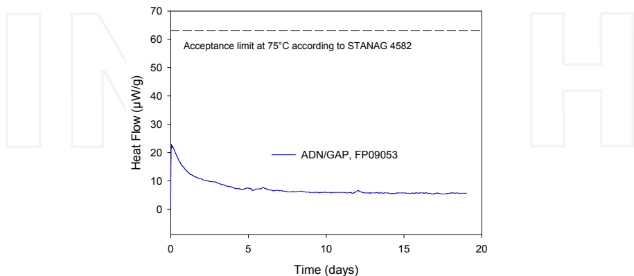
Fig. 7. Thermal stability at 75^\circ\text{C} of ADN/GAP propellant containing 70 % ADN.
