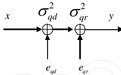
Fig. 12. Equivalent representation of the noisy quantization for a fixed input signal. The input signal determines the parameters \sigma_{qd}^2 and \sigma_{qr}^2 .
