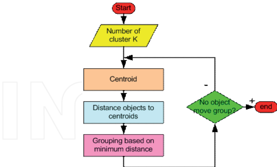
Fig. 3. K-means iteration
