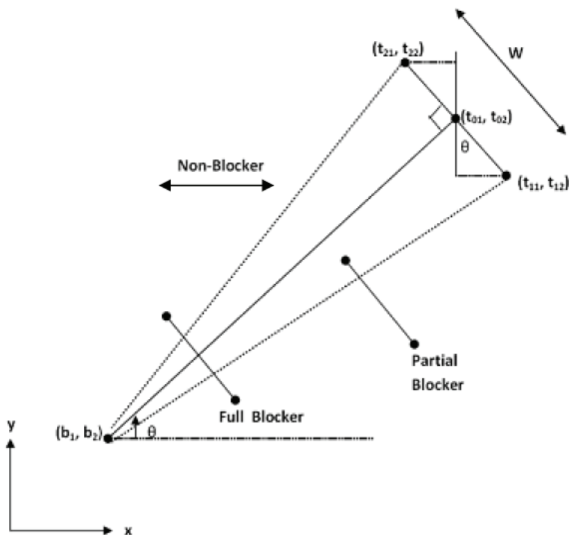
Fig. 6. Full, partial and no blockers in 2D
