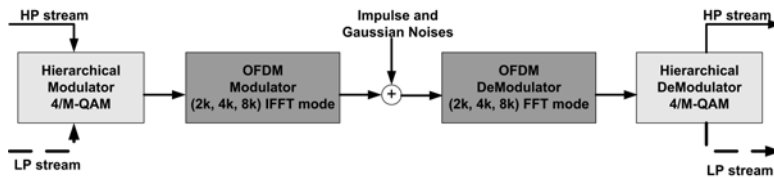
Fig. 5. Simulated block diagram of OFDM hierarchical QAM system
