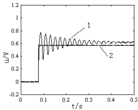
Fig. 6-29 Input and nonlinear output (1)nonlinear output, (2) input signal
