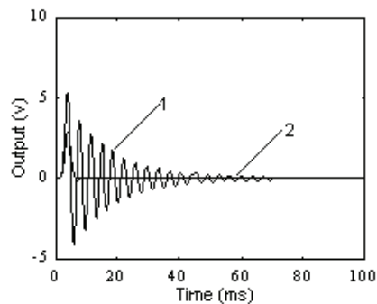
Fig. 6-15 The first step of compensation (1) nonlinear dynamic response, (2) dynamic compensation of the first step.
