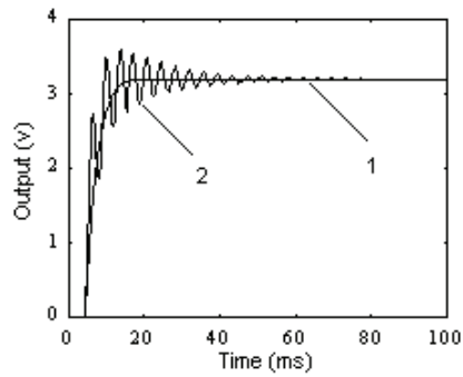
Fig. 6-13 The first step of compensation: (1) nonlinear dynamic response, and (2) dynamic compensation of the first step.
