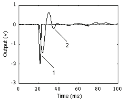
Fig. 6-8 Impulse response in HLC: (1) impulse input, and (2) dynamic response of the sensor.
