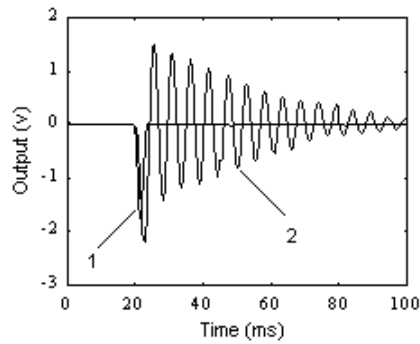
Fig. 6-7 Impulse response in NLC: (1) impulse input, and (2) dynamic response of the sensor.
