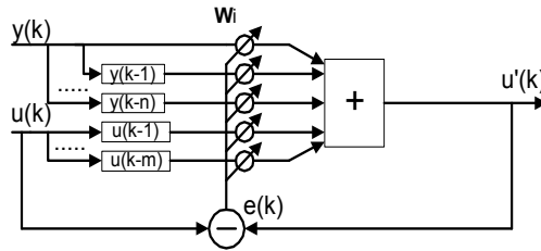
Fig. 4-1 Design schematic of dynamic compensating device by FLANN
