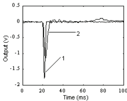
Fig. 6-17 Compensation result of NLC compared with the input signal (1) impulse input, (2) nonlinear dynamic compensation result
