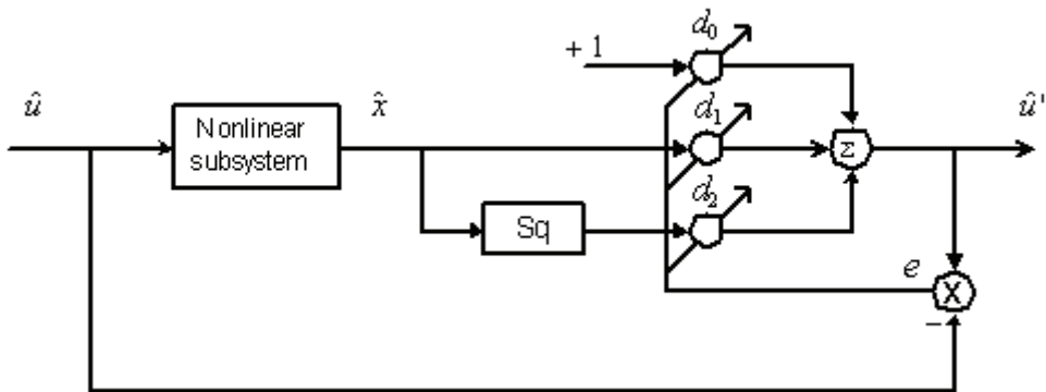
Fig. 6-12 A training schematic diagram of the FLANN
