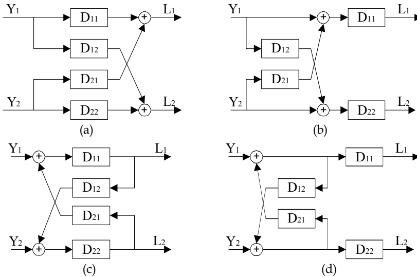
Fig. 5-1 Four kinds of network structures
