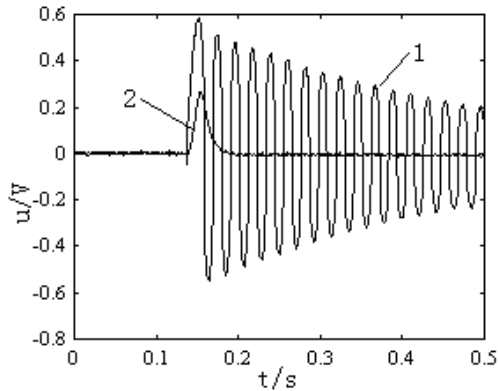
Fig. 6-33 Nonlinear output and compensation result (1) nonlinear output, (2) compensation result
