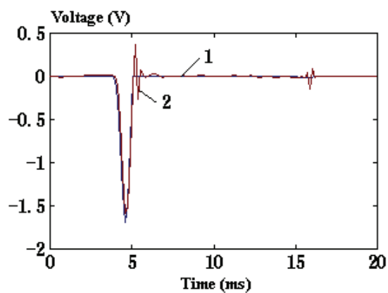
Fig. 5-4 (a) Decoupling and compensating result of direction Z
