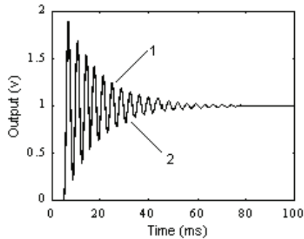
Fig. 6-2 Comparison of two response curves: (1) step response of Equ.(6-7), and (2) step response of Equ.(6-16).
