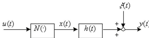
Fig. 6-1 Hammerstein model
