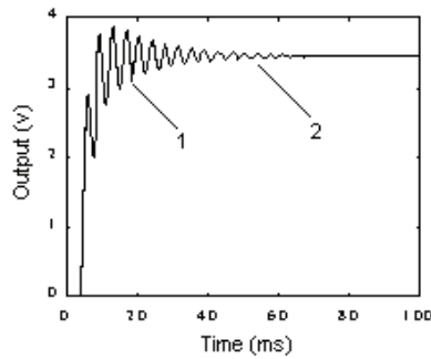
Fig. 6-4 Comparison of identification result and supposed response: (1) supposed response, and (2) identification result.
