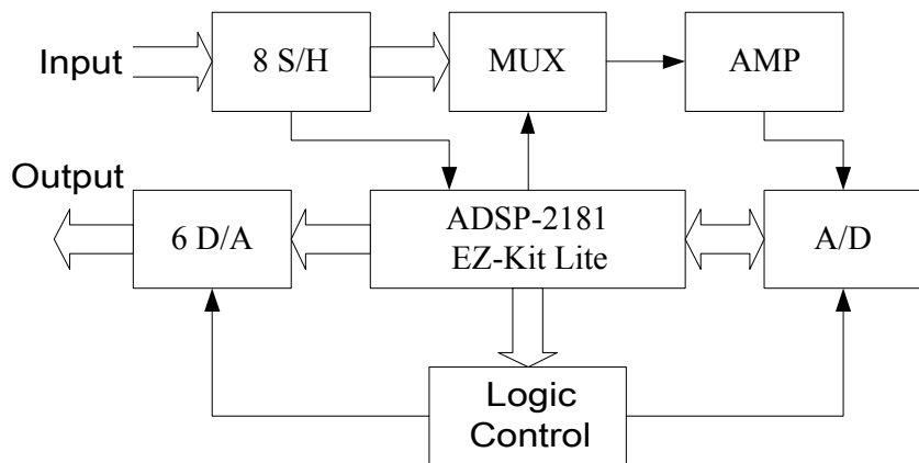
Fig. 4-2 Schematic block diagram of dynamic compensating system
