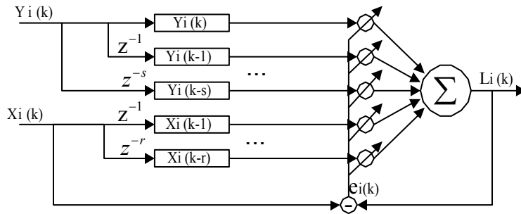
Fig. 5-2 Schematic of modeling by FLANN
