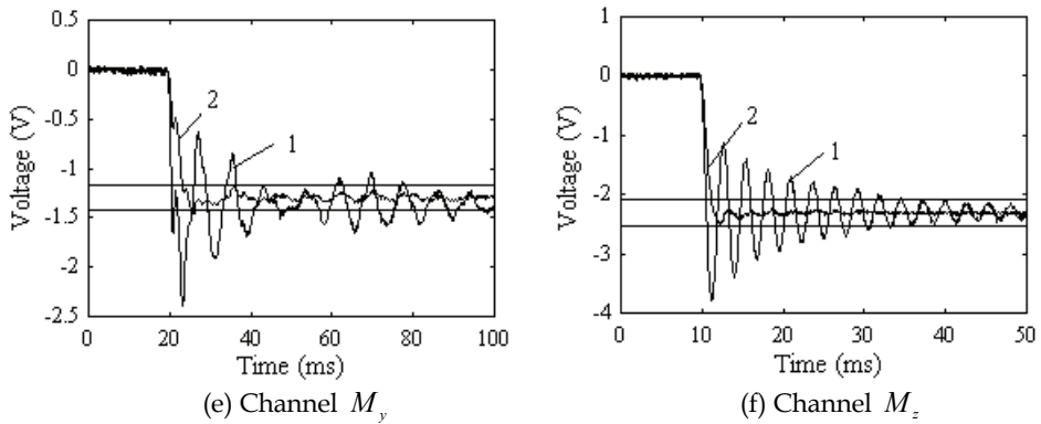
Fig. 4-3 Experiment results (1) dynamic response of sensor, (2) output of dynamic compensating system.
