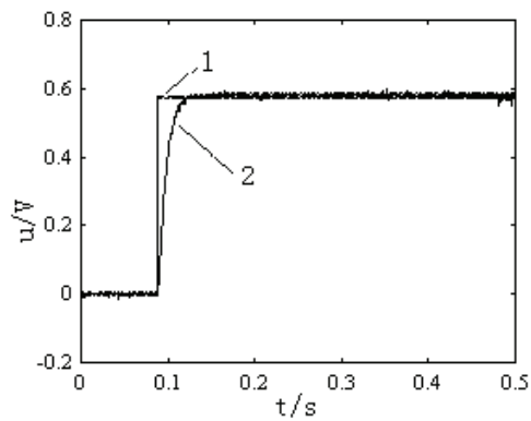
Fig. 6-30 Nonlinear output and compensating result (1) input signal, (2) compensated result
