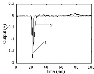
Fig. 6-18 Compensation result of NLC using linear approach compared with the input signal (1) impulse input, (2) compensation result
