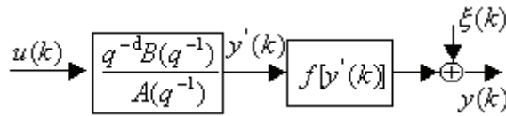
Fig. 6-21 Structure scheme of sensor after decomposition
