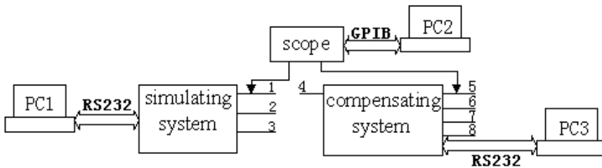
Fig. 6-28 Experimental setup
