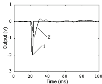
Fig. 6-20 Compensation result of HLC using linear approach compared with the input signal (1) impulse input, (2) compensation result
