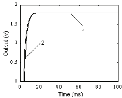
Fig. 6-14 The second step of compensation compared with the input signal (1) step input, (2) nonlinear static correction of the second step.
