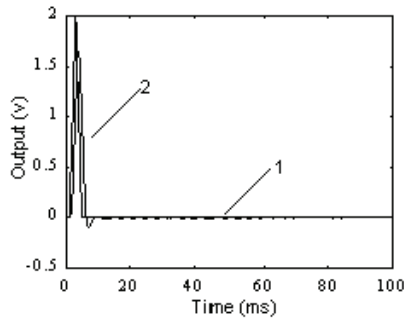
Fig. 6-16 The second step of compensation compared with the input signal (1) impulse input, (2) nonlinear static correction of the second step.
