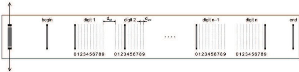
Fig. 5. Practical example of time position encoding. (Stelzer et al., 2004)
