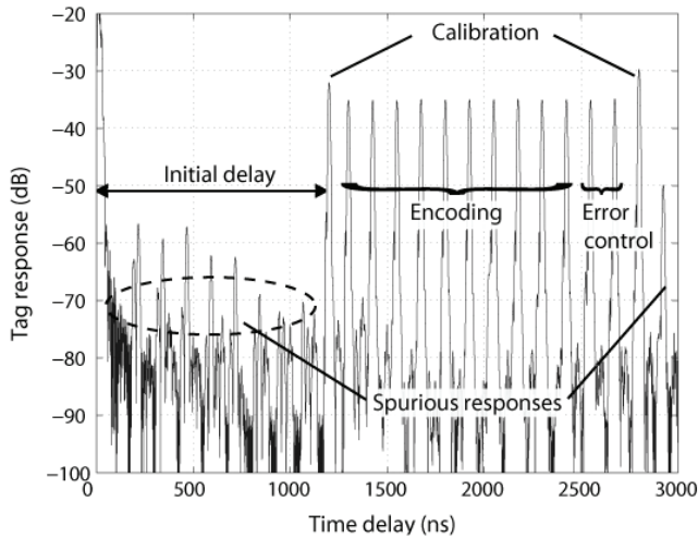
Fig. 2. Simulated SAW tag response.
