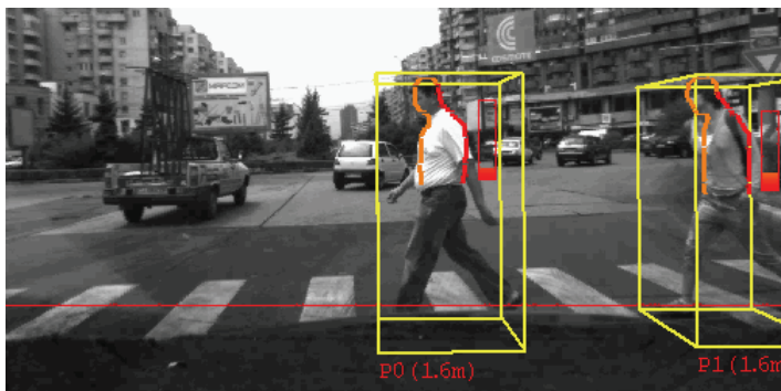
Fig. 20. Detected pedestrians
