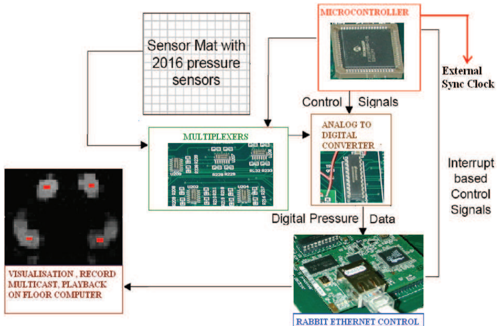
Fig. 3. System level block diagram of the mat-based controller
