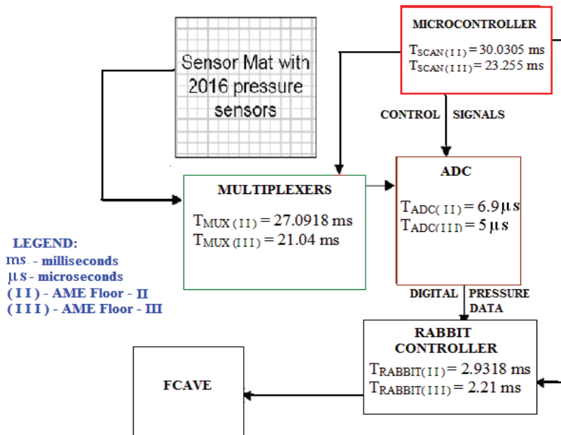
Fig. 8. Block diagram of Floor hardware annotated with hardware component delays
