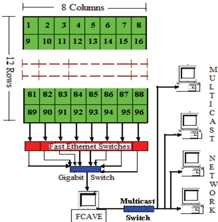
Fig. 2. Floor System overview and related network architecture
