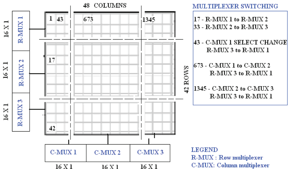
Fig. 9. The arrangement of multiplexers for a pressure sensing mat and sensors that require longer scanning time due to multiplexer switching.
