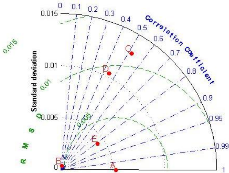
Figure 12. Taylor diagram showing the comparison under different prior hypotheses on roughness. A refers to ground measurements; B to low roughness; C to high roughness; D to whole range of roughness; E adapted roughness ranges.
