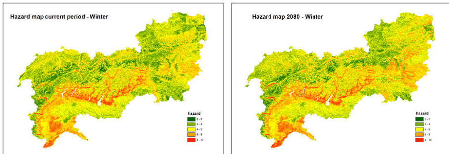
Figure 12. Alpine Space, maps of winter hazard (2011 - 2080)
