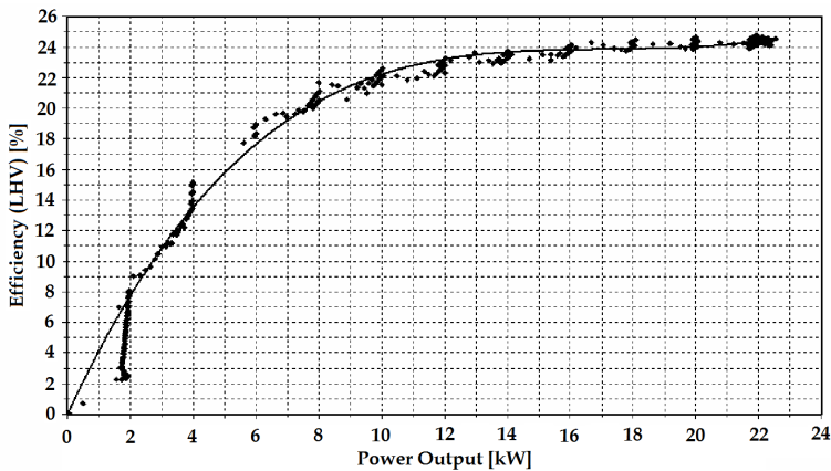
Figure 15. Microturbine efficiency at partial loads
