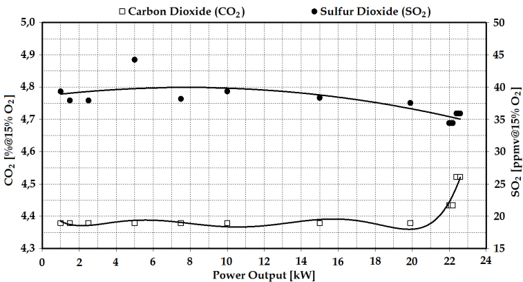
Figure 17. CO 2 and SO 2 emissions from liquid fuel microturbine at partial loads.
