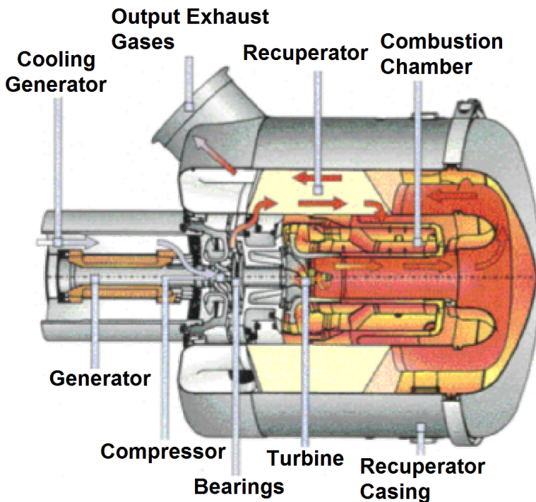
Figure 6. Parts of a Capstone microturbine.
