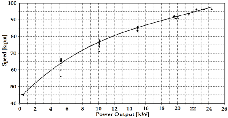
Figure 9. Microturbine speed at partial loads.
