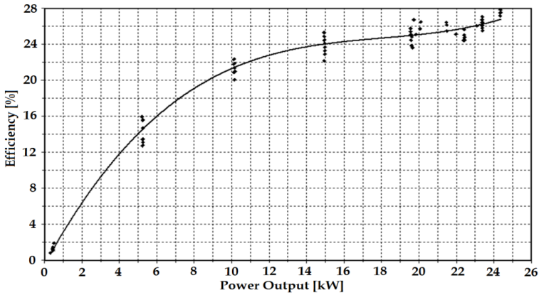
Figure 11. Microturbine efficiency at partial loads.
