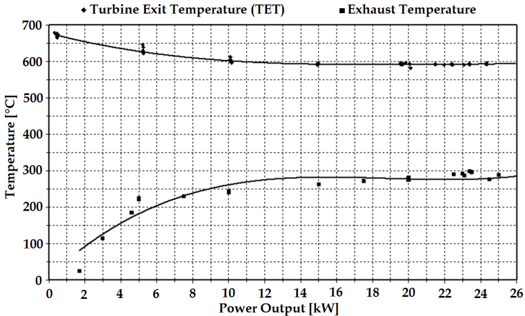
Figure 10. Microturbines exhaust temperature at partial loads.
