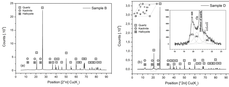
Figure 12. The XRD pattern of Sample B (a) and Sample D (b).
