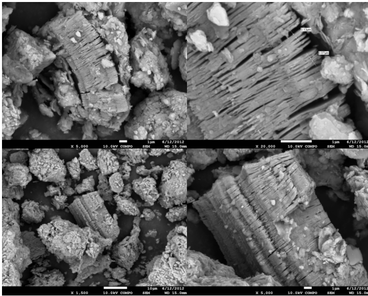
Figure 10. Clay from termite nest (Sample D).
