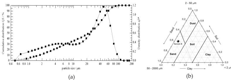
Figure 7. The granulometry of the Sample D (a) and total granulometric composition (b).
