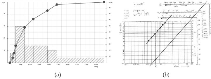
Figure 6. The sieve analysis of the Sample C (a) and RRSB diagram (b)
