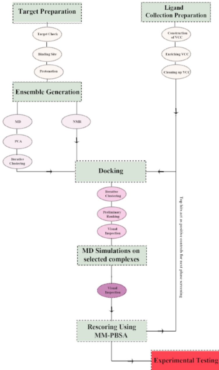
Figure 4. The implemented virtual screening protocol.
