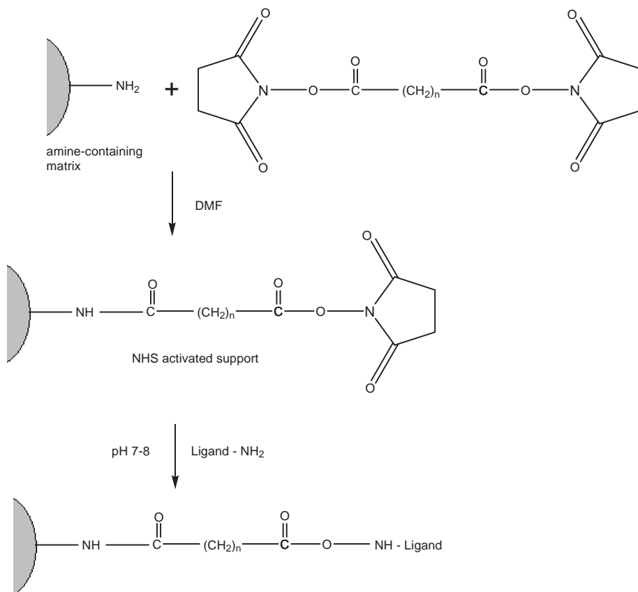
Figure 13. N-Hydroxysuccinimide immobilization method [8]
