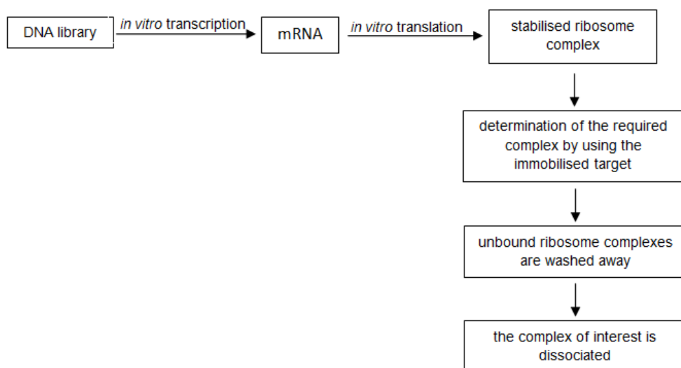
Figure 9. Ribosome display method [9]
