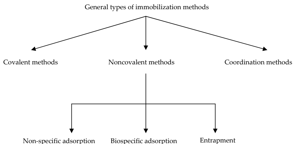
Figure 11. Immobilization methods used in affinity chromatography
