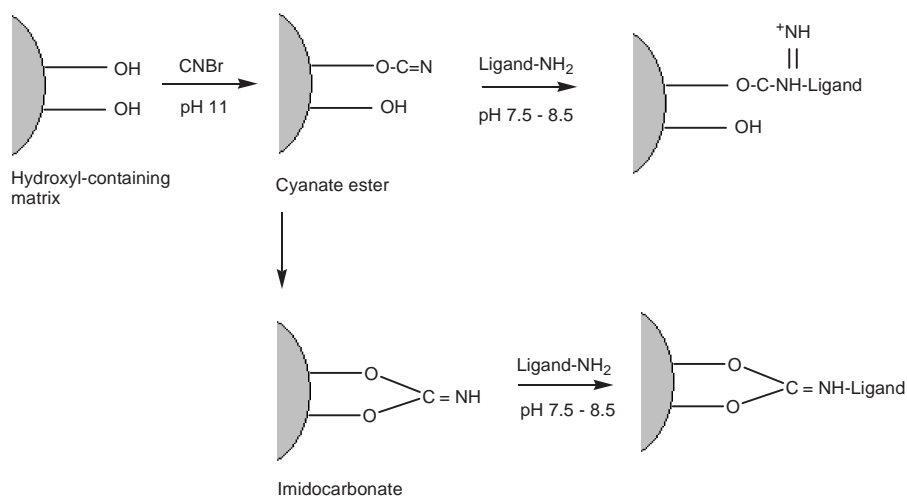
Figure 12. Cyanogen bromide immobilization method pathway [8]
