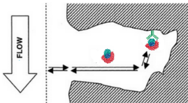
Figure 6. Transport processes that occur in a chromatographic column.
