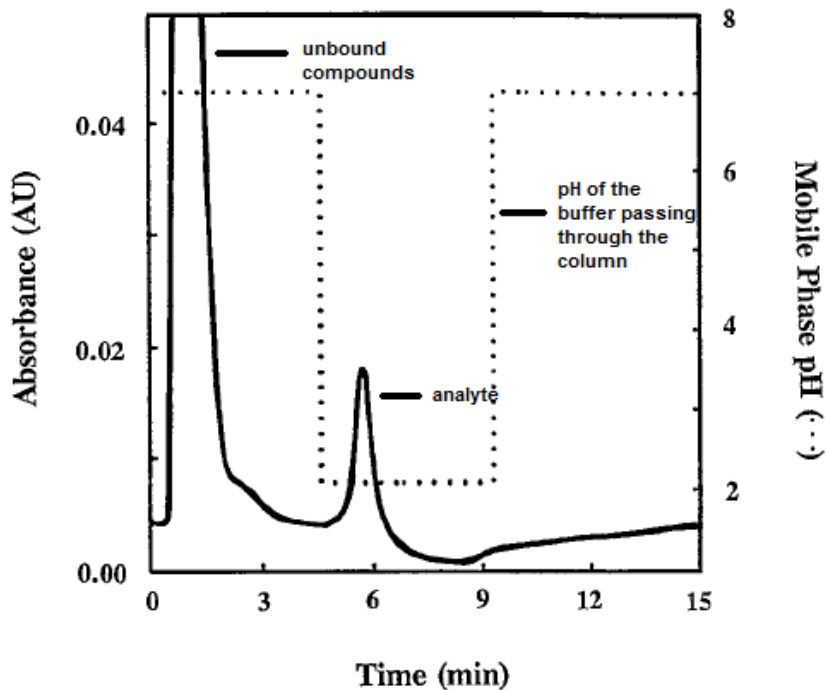
Figure 2. An example of a typical scheme of an affinity chromatography application [1].
