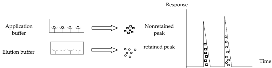
Figure 15. Typical separation in affinity using step gradient elution.
