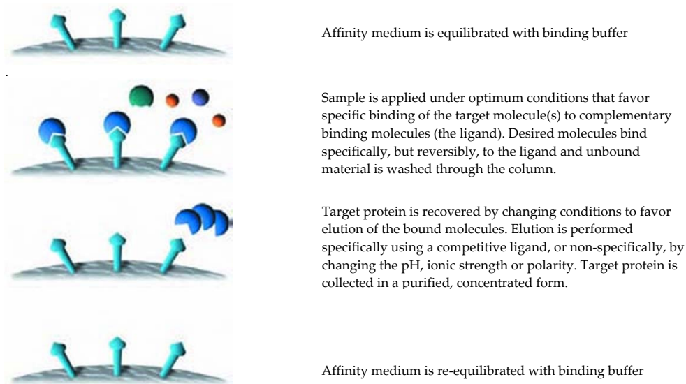
Figure 1. Separation procedure in affinity chromatography
