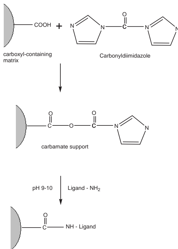
Figure 14. The carbonyldiimidazole immobilization method [8]
