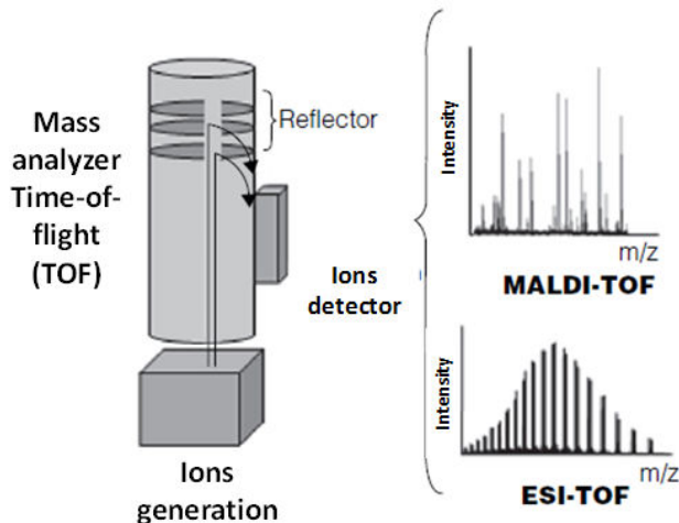
Figure 4. Scheme of Mass Spectrometer. Mass analyzer characterized and separated ions according to their mass/charge ratio ( m/z ). Ions detector generate mass spectrum for every ion detected. MALDI and ESI mass spectrum obtained are shown.
