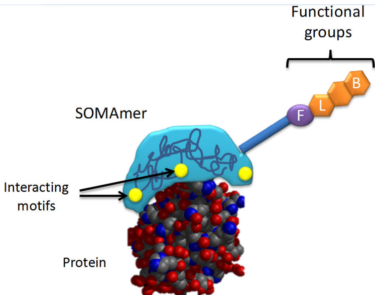
Figure 2. SOMAmer-protein complex. SOMAmer binds specifically to protein target through interacting motifs. Functional groups are: B= biotin for capture; F=Cy3 for detection and L=photocleavable linker.
