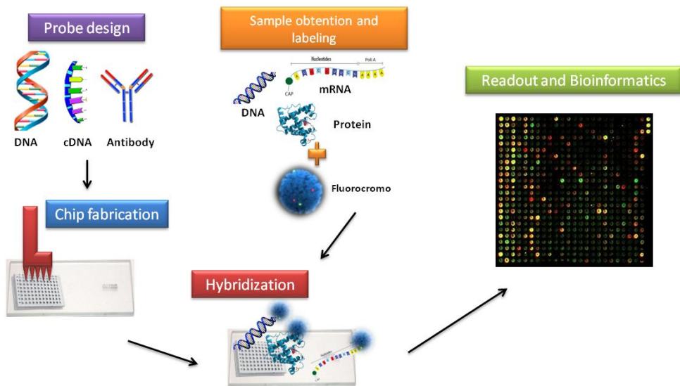
Figure 1. Design and implementation of DNA microarray experiment
