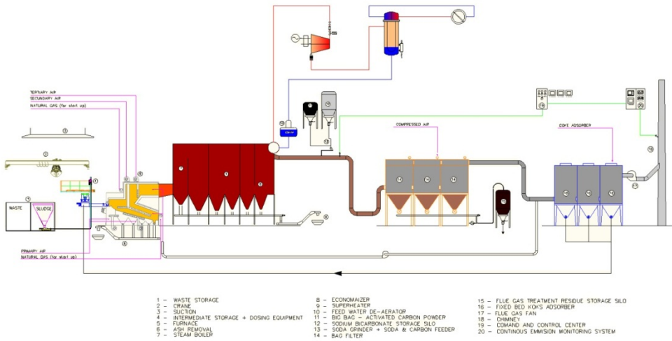
Figure 9. Schematic presentation of W-t-E plant
