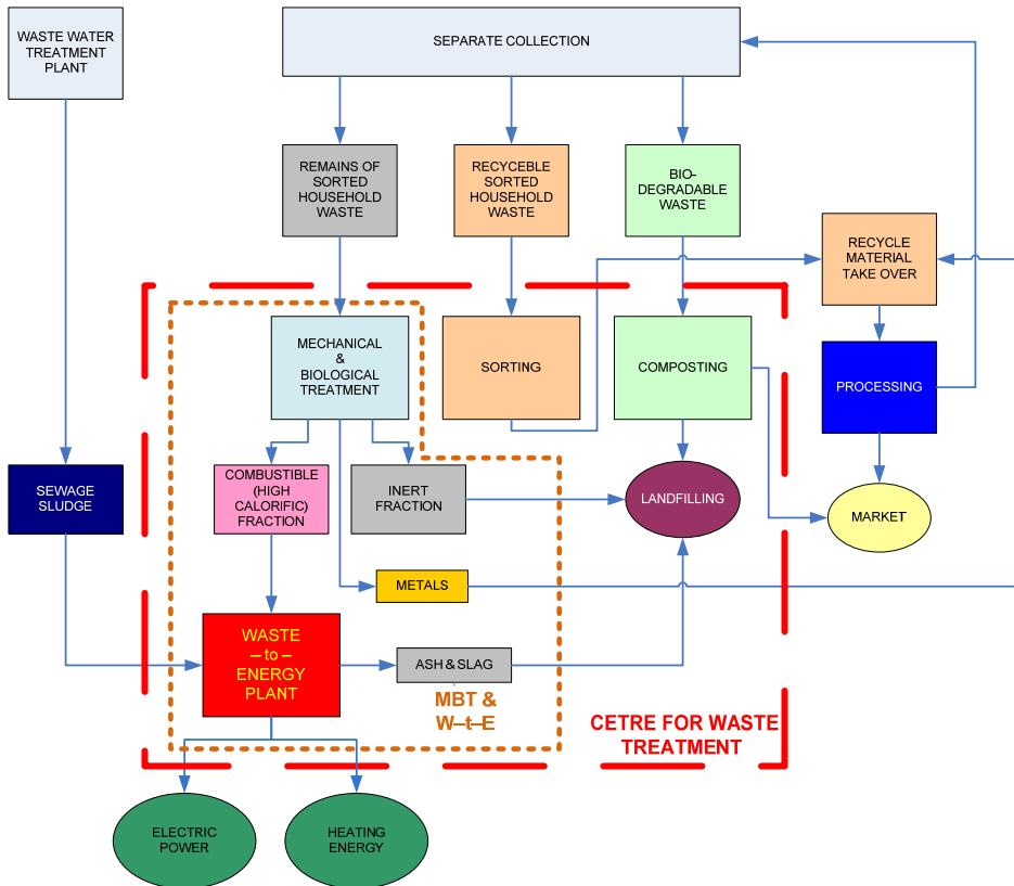
Figure 1. Schematic presentation of integrated waste management concept
