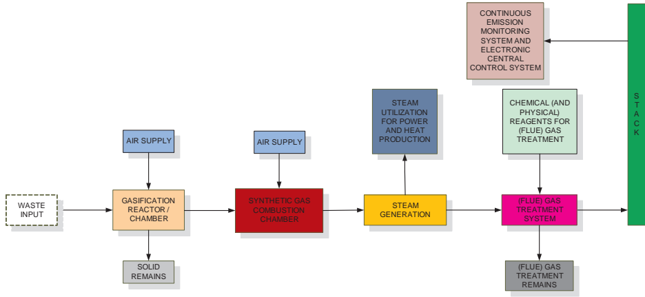
Figure 5. The schematic presentation of complete waste gasification system with immediate combustion of synthetic gas
