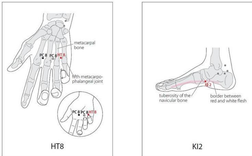
Figure 7. Location of selected acupuncture points for tonification of heart fire – HT8 is used to generate warmth by tonification of the heart fire and KI2 is used to generate warmth by tonification of the kidney fire. The selection of acupuncture points located were based on the publication of WHO standard acupuncture point locations.
