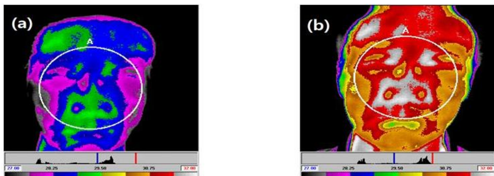
Figure 10. Facial temperature before and after treatment with a real needle -The changes in facial temperature after smoking (a) and after being treated by real needle (b). After treatment with a real needle, the average facial temperature shows an overall increase. On the color bar below the photos, higher temperatures are located on the right.
