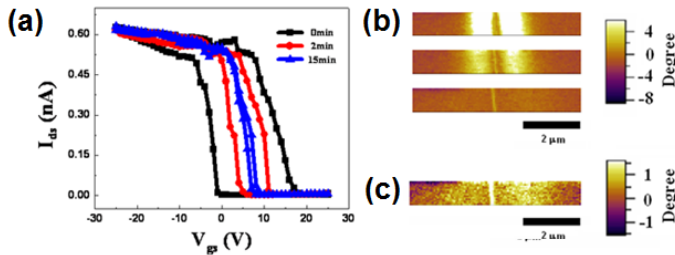
Figure 11. Hysteresis-free transfer curve under ambient condition. (a) Hysteresis width can be reduced by allowing the injected charges to dissipate at every gate bias. The experiment was conducted by turning the gate bias off at every step for 0 (black), 2 (red) and 15 (blue) minutes, and measure the I_{ds} immediately after turning the gate bias back on. (b) The corresponding EFM images after 0 (top), 2 (middle) and 15 (bottom) minutes discharging time. (c) The bottom image in (b) replotted with reduced scale. A small amount of injected charges is observed. Reprinted with permission from [40] Copyright 2012, IOP Publishing.
