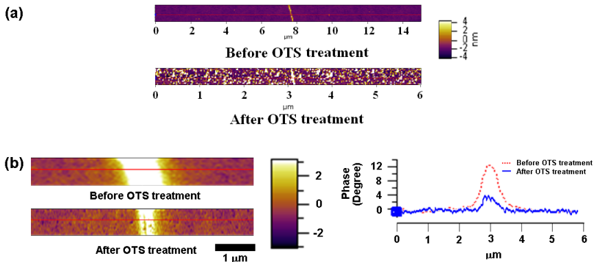
Figure 15. Surface modification with OTS (a) Topography images of sample before and after OTS treatment for 72 hrs. (b) Corresponding EFM images of (a) after charging with -5 V bias. (c) Cross section profiles of EFM images clearly shows the decrease in injected charges.
