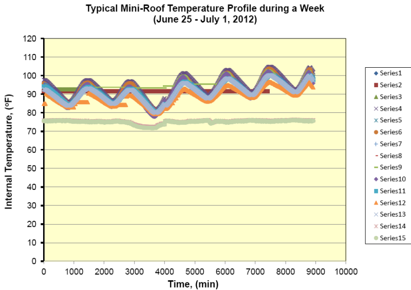
Figure 10. Typical internal mini-roof temperatures during the course of a week.
