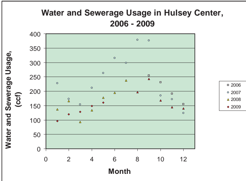
Figure 22. Water/wastewater usage for operation of Hulsey Center, 2006 – 2009.
