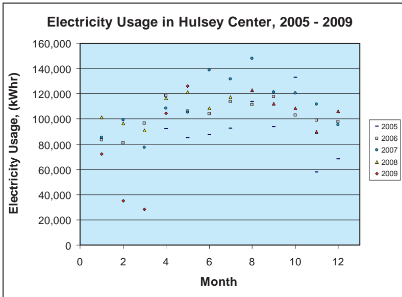
Figure 23. Electricity usage for operation of Hulsey Center, 2005 – 2009.
