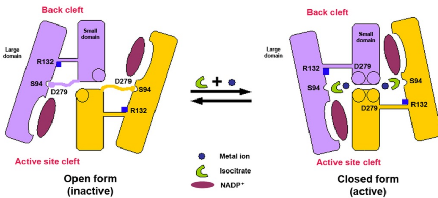
Figure 2. Structure of the wild-type IDH1 homodimer.
