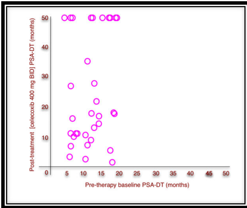
Figure 11. Smith et al. [79] studied the biologic activity of celecoxib, a selective cyclooxygenase-2 inhibitor, in men with recurrent prostate cancer using change in PSA-DT as the primary outcome variable. We retrieved their graphic data for our own analysis. A histogram of the PSA-DT paired differences for before and after celecoxib appears normally distributed. Applying the parametric Paired t-test statistic for significance of the difference yields p = 0.0002 . Next, we transformed the same (before-after celecoxib PSA-DT data with to PSA-SGR before and after pairs and applied the paired t-test. Contrary to the statistical analysis for celecoxib induced change of PSA-DT, changes of PSA-SGR revealed that the celecoxib difference was no longer significant, p = 0.213!
