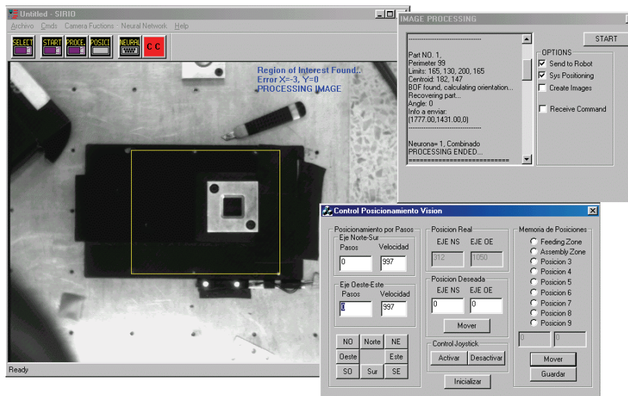
Figure 9. SIRIO main screen
