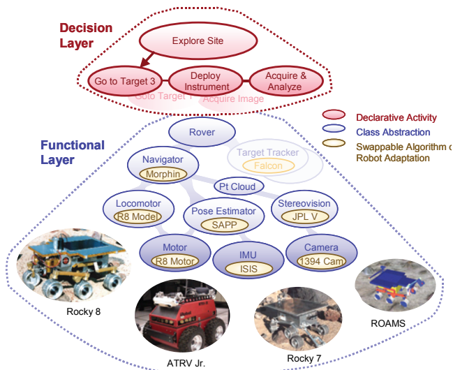
Fig. 1. The CLARAty Architecture
