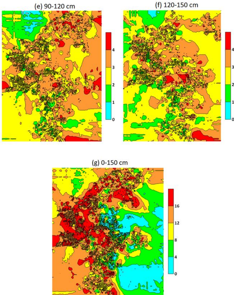
Figure 8. Digital soil mapping of the estimated SOC stock at different depth in arable soils of Tainan (unit: \text{kg m}^{-2} ). Cross symbols represent the soil sampling pedons. Each pedon was sampled by auger within a 250 m by 250 m grid (6.25 ha).
