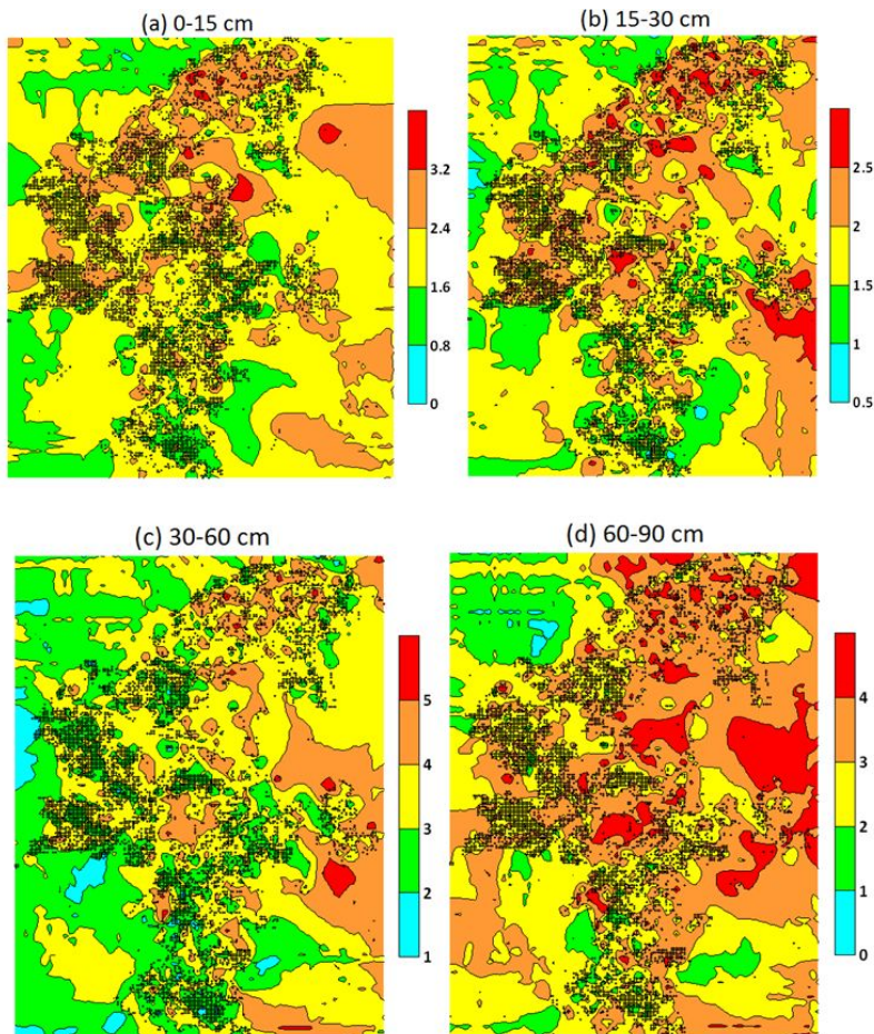
Figure 8. Digital soil mapping of the estimated SOC stock at different depth in arable soils of Tainan (unit: \text{kg m}^{-2} ). Cross symbols represent the soil sampling pedons. Each pedon was sampled by auger within a 250 m by 250 m grid (6.25 ha).
