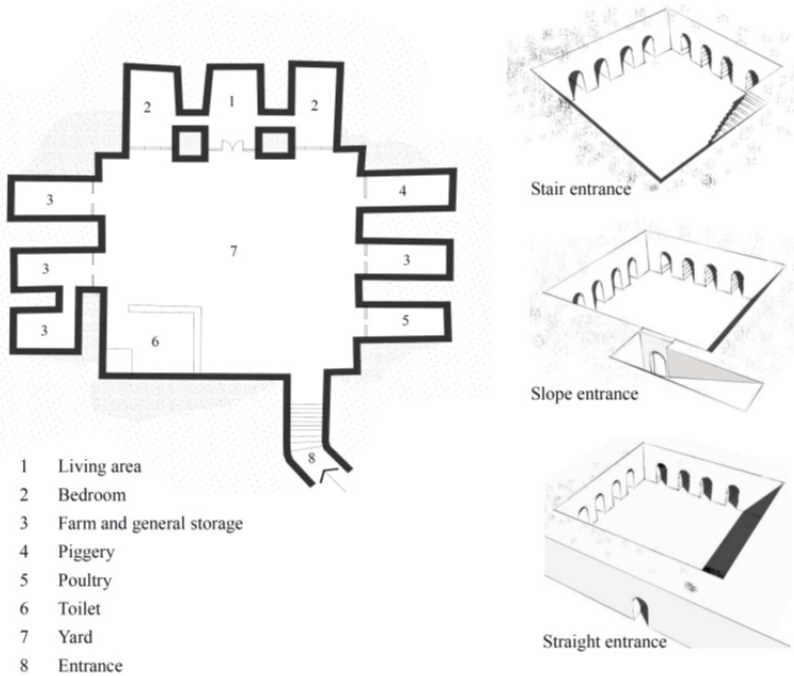
Figure 4. A typical earth shelter home layout in North-western China
