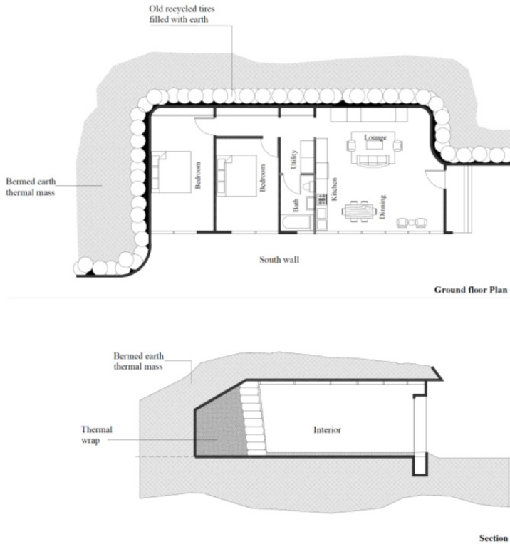
Figure 6. An Earth Ship design, using recycled materials
