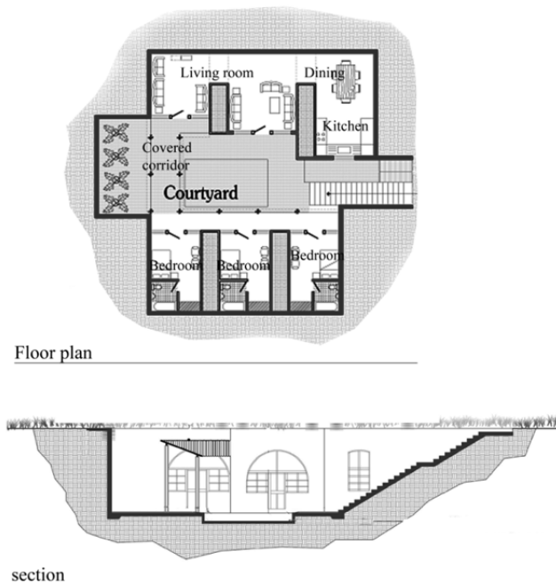
Figure 8. Underground earth shelter design
