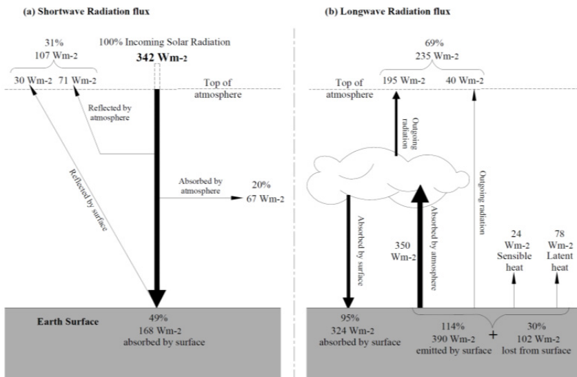
Figure 10. Earth’s energy budget diagram showing the short-wave (a) and long-wave (b) energy fluxes
