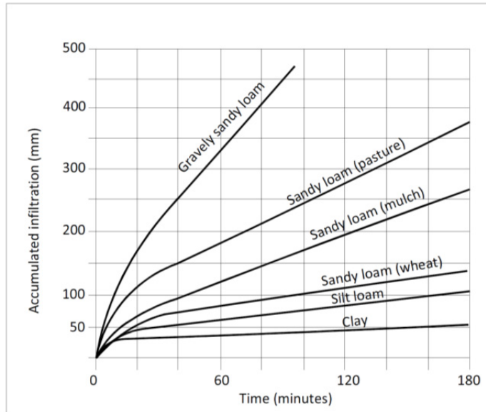
Figure 13. Infiltration curves for different soil textures
