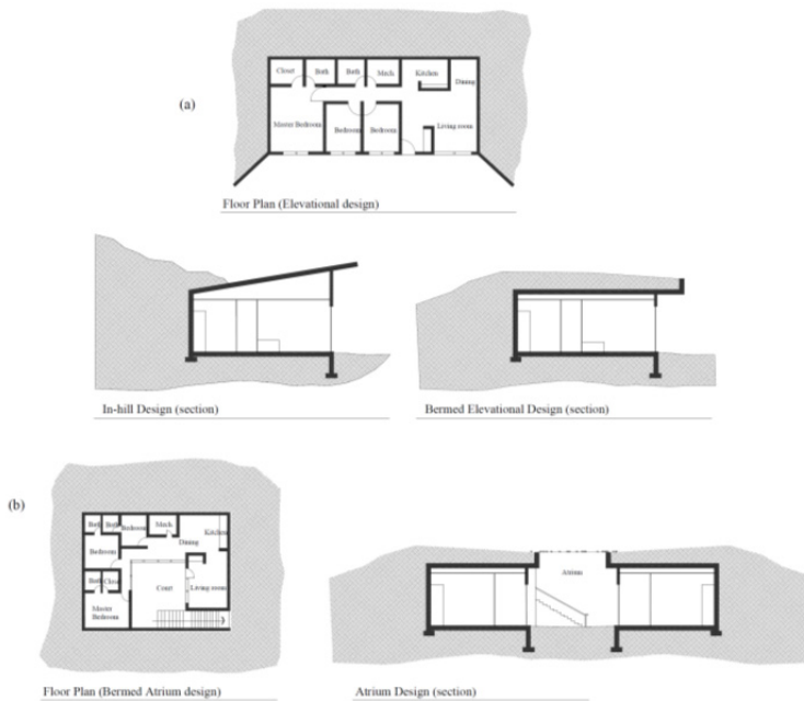
Figure 7. (a) Elevational (bermed) and in-hill designs, (b) Atrium (bermed) design
