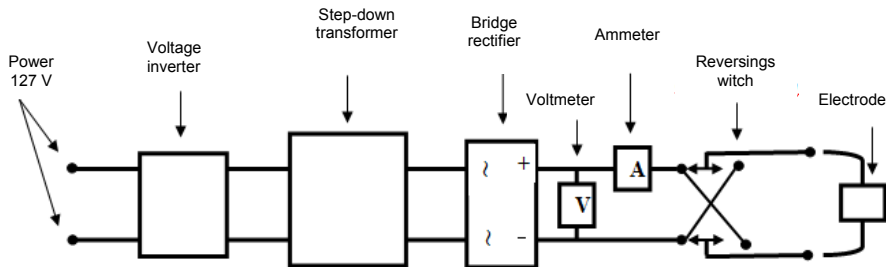
Figure 4. Schematic diagram of the experimental DC unit.
