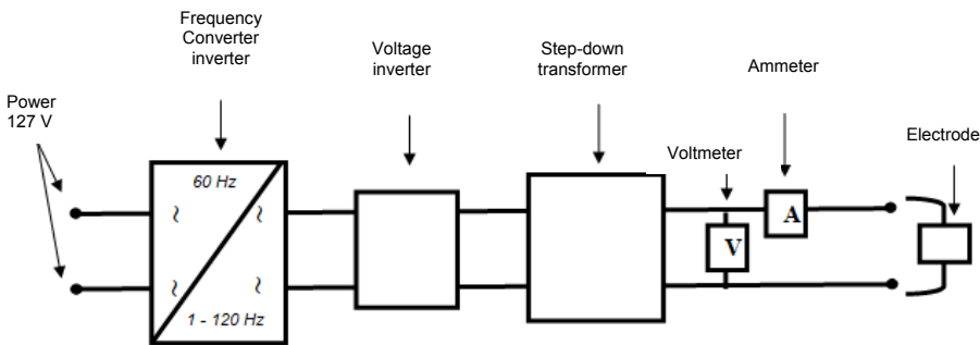
Figure 5. Schematic diagram of the experimental AC unit
