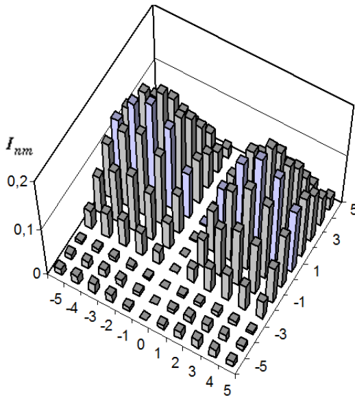
Figure 9. Optimal distribution of current on the radiators, which creates the branching solution
