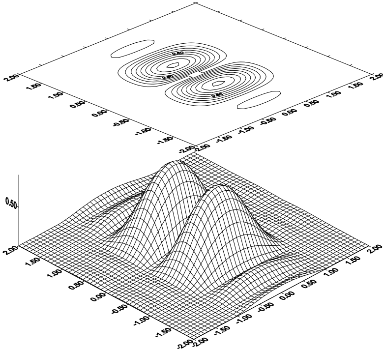
Figure 8. Amplitude directivity pattern of solution branched off from f_0(\xi_1, \xi_2, c_1, c_2)
