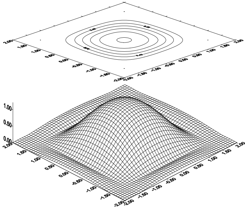
Figure 1. Amplitude directivity pattern of a trivial solution f_0(\xi_1, \xi_2, c_1, c_2)
