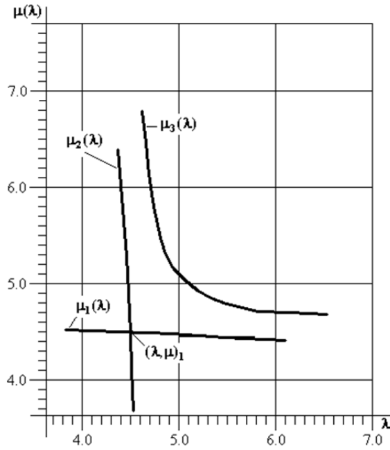
Figure 13. Eigenvalue curves for F(\xi_1, \xi_2) = \cos \frac{\pi}{2} (\sqrt{\xi_1^2 + \xi_2^2})
