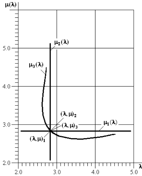
Figure 10. Eigenvalue curves for F(\xi_1, \xi_2) = 1
