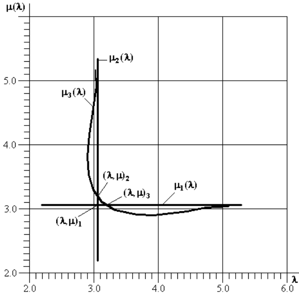
Figure 12. Eigenvalue curves for F(\xi_1, \xi_2) = \sqrt{1 - (\xi_1^2 + \xi_2^2)} / 2
