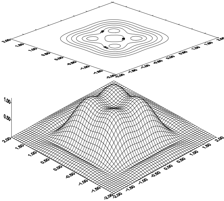
Figure 3. Amplitude directivity pattern of the solution branched from f_0(\xi_1, \xi_2, c_1, c_2)
