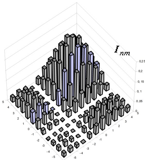
Figure 4. Optimal current distribution on radiators, which creates the branched solution
