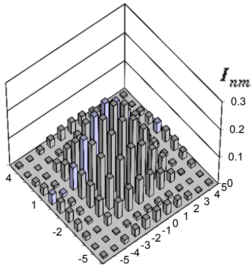
Figure 2. Current cophasal distribution on the radiators, which creates the diagram f_0(\xi_1, \xi_2, c_1, c_2)
