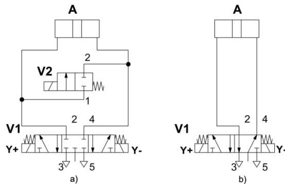
Figure 7. Pneumatic circle a) with restoring energy, b) without restoring energy (Blagojević et al., 2011)
