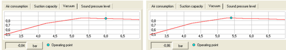
Figure 6. Vacuum level at operating pressure of 6 bar (left) and 5.4 bar (right)
