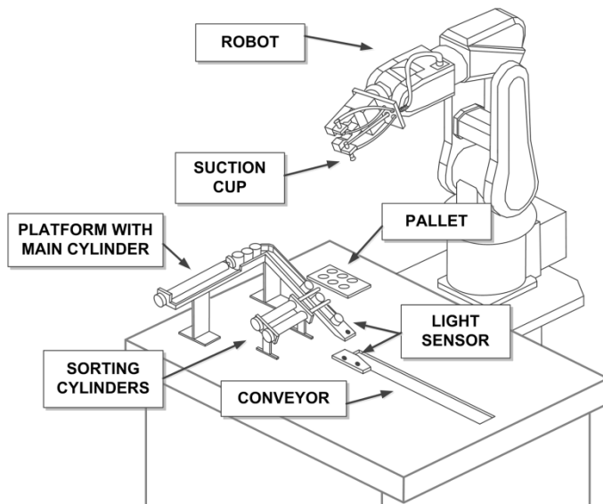
Figure 8. Complex robotic cell
