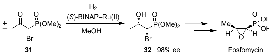
Scheme 16. Synthesis of fosfomycin via dynamic kinetic resolution
