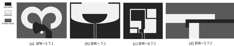
Figure 18. Special geometries of wide-slot antennas [49-52].
