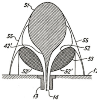
Figure 3. Schelkunoff's spherical dipole (1940)
