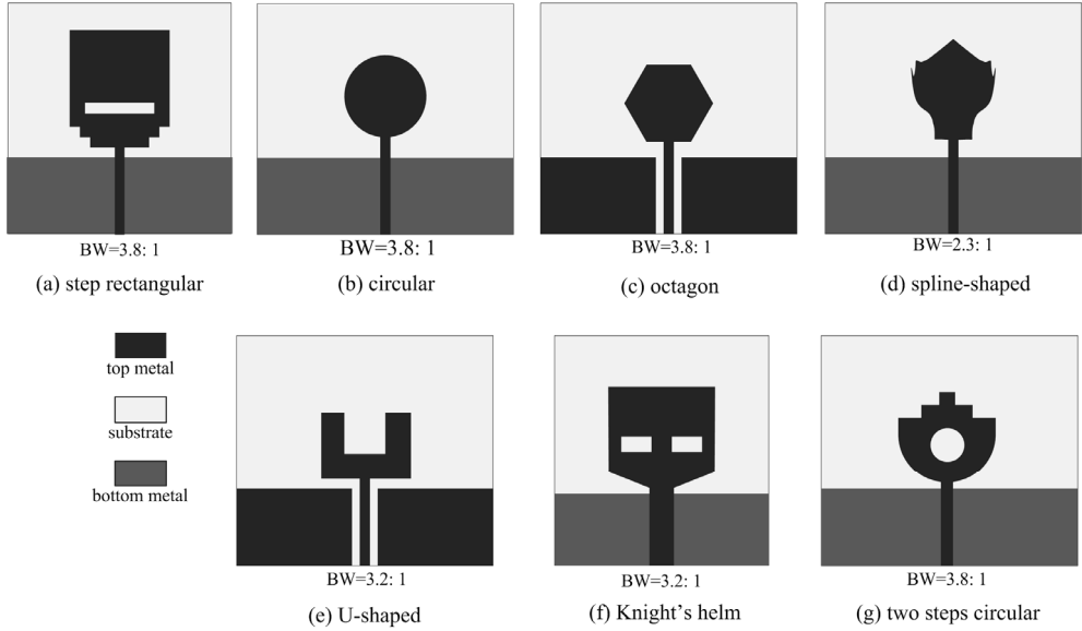
Figure 11. Various monopole structures [21-27].
