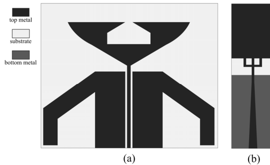
Figure 14. Radiation improvement techniques [37, 38].
