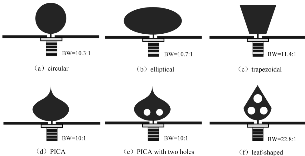
Figure 9. Various geometries of planar monopole antennas [11-14] .
