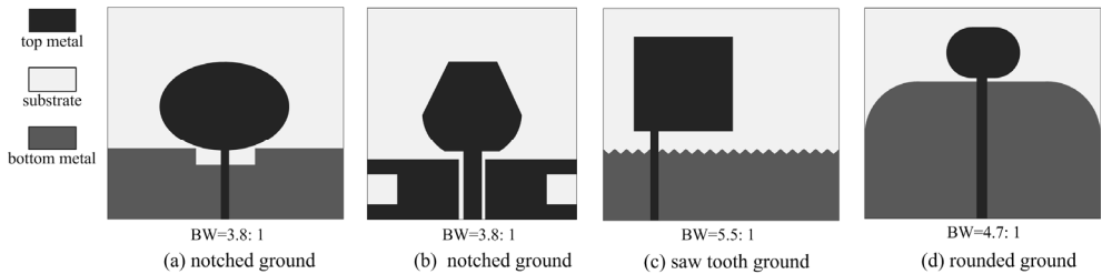
Figure 12. Various ground structures [28-31].
