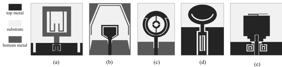
Figure 30. Hybrid notched-band techniques [83-87].
