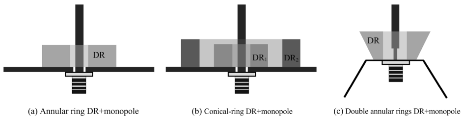
Figure 22. UWB hybrid DRAs [54-56].
