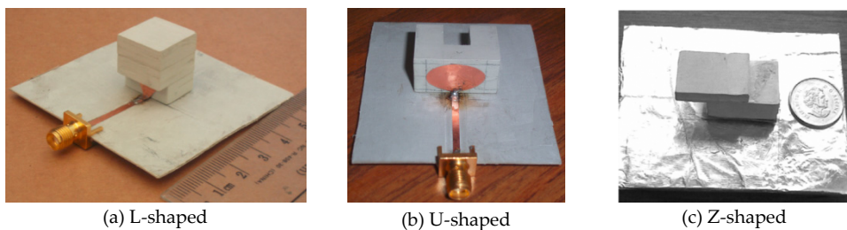
Figure 23. Photos of various UWB DRAs [58-60].
