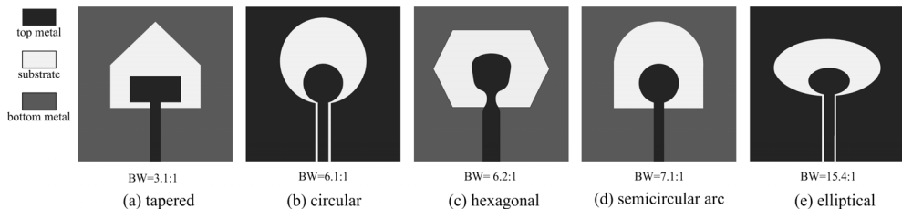
Figure 17. Various shapes of wide-slots [44-48].
