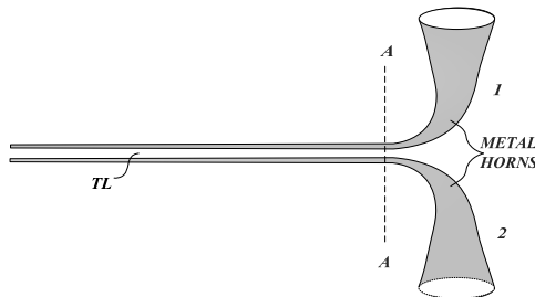
Figure 2. Carter’s improved match biconical (1939).
