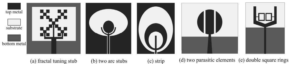
Figure 28. Notched-band designs with various stubs [74-78].
