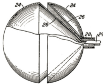
Figure 3. Schelkunoff's spherical dipole (1940)
