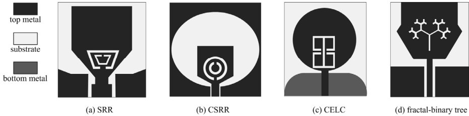
Figure 27. Notched-band designs with various periodic structure slots [70-73].
