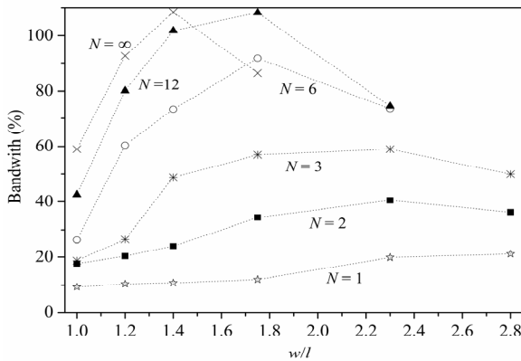
Figure 21. Various bandwidths for orders N .
