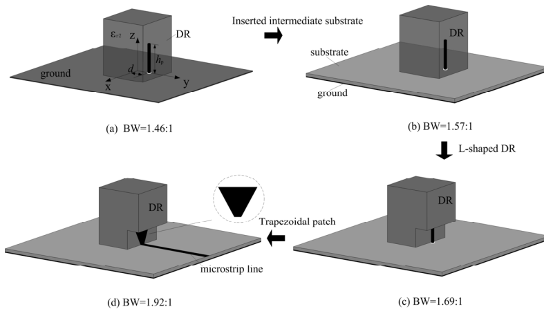
Figure 24. Wideband DRA design.
