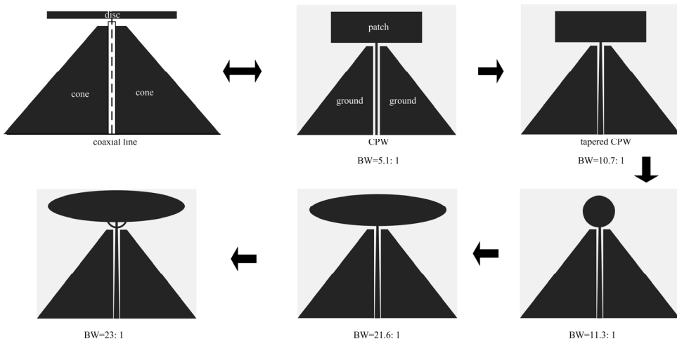
Figure 13. Various printed monopole antennas with trapeziform ground [32-36].
