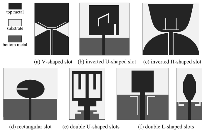
Figure 26. Notched-band designs with various slots on patch or ground [63-69].
