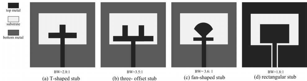
Figure 16. Various shapes of tuning stubs [40-43].
