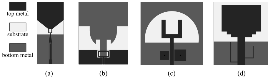
Figure 29. Various bandstop transmission lines [79-82].
