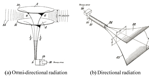
Figure 6. Brillouin's coaxial horn (1940).
