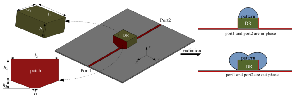
Figure 25. UWB DRAs with a radiation reconfiguration.
