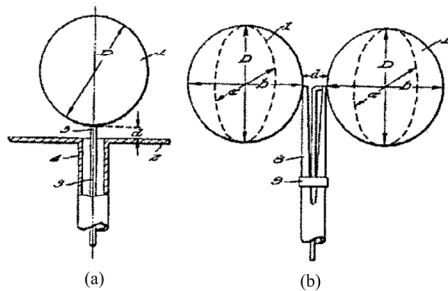
Figure 8. Stohr's ellipsoidal monopole and dipole (1968).
