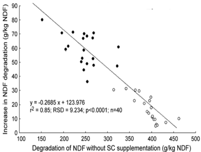
Figure 4. Figure 4. Effects of supplementation with a yeast probiotic ( Saccharomyces cerevisiae CNCM I-1077) on fibre (NDF) degradation of maize silages after 36h of incubation in the rumen of cows: open circles, high fibre degradation group, full circles, low fibre degradation group. From [85].
