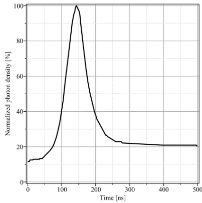
Figure 9. Measured first laser pulse time-shape.
