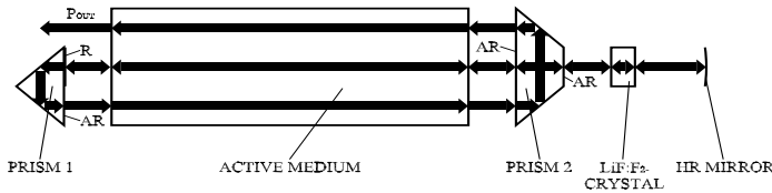
Figure 5. Schematic representation of the slab laser setup. PRISM 1, PRISM 2 – prisms; R – 53 % reflective coating as output coupler; AR – anti-reflective coating; LiF:F 2 CRYSTAL – passive optical Q-switch cell; ACTIVE MEDIUM – Nd:YAG slab; HR MIRROR – high reflectivity mirror; P out – outgoing laser beam.
