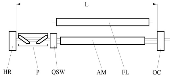
Figure 2. Schematic representation of the rod laser setup. HR - high reflectivity back mirror; P - polarizer; QSW – LiF:F 2 passive optical Q-switch cell; AM – active medium; FL – flash lamp; OC – output coupler; L – optical resonator length
