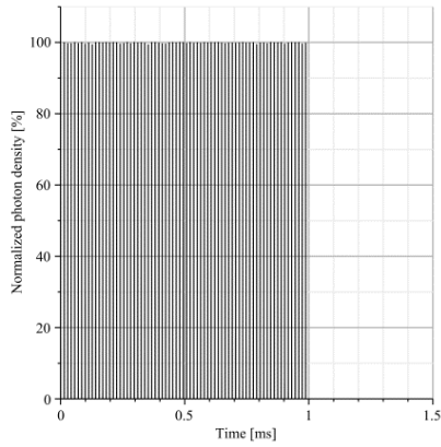
Figure 6. Simulated laser pulses train time-shape.
