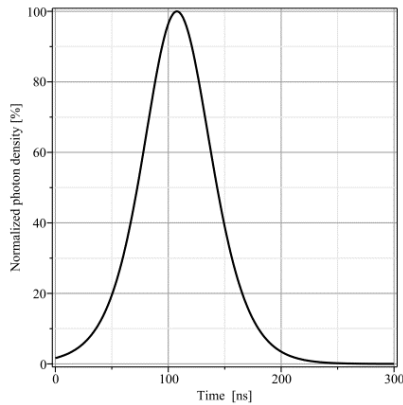
Figure 8. Simulated single laser pulse time shape.
