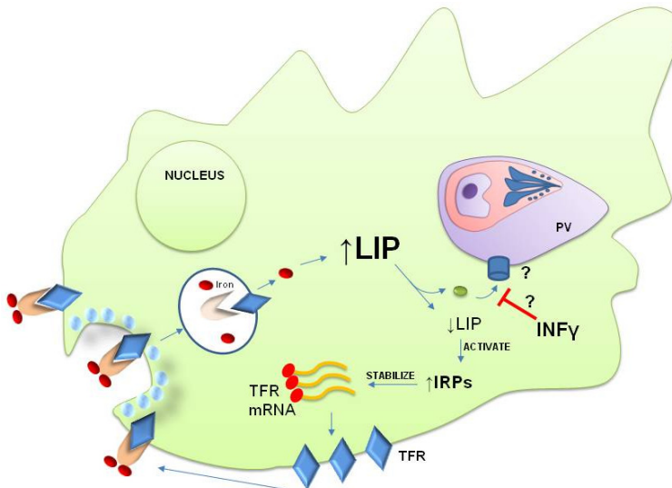
Figure 7. Iron uptake by intracellular Toxoplasma gondii . T. gondii lives inside a parasitophorous vacuole (PV) within the host cell; from there, it sequesters iron \bullet and depletes the macrophage labile-iron pool (LIP), activating the host cytosolic iron-responsive element sensor proteins (IRPs). These proteins increase the stability of the TFR mRNA \bullet , increasing host cell iron uptake from TF \bullet . This positive regulation system increases the intracellular iron that the parasite requires for survival. Iron uptake by the parasite is limited by TNF \gamma through an unknown mechanism.
