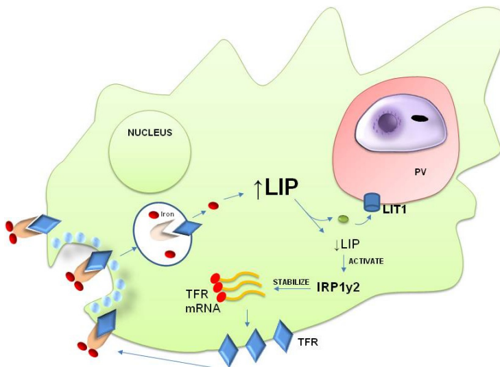
Figure 6. Iron uptake by intracellular Leishmania donovani amastigotes. From its parasitophorous vacuole (PV), Leishmania expresses its ferrous iron transporter (LIT1) to scavenge iron and deplete the macrophage labile-iron pool (LIP); this activates the host cytosolic iron-responsive element sensor proteins IRP1 and IRP2. These proteins increase the stability of the TFR mRNA, increasing macrophage iron uptake from TF and the intracellular iron parasite needs for survival.
